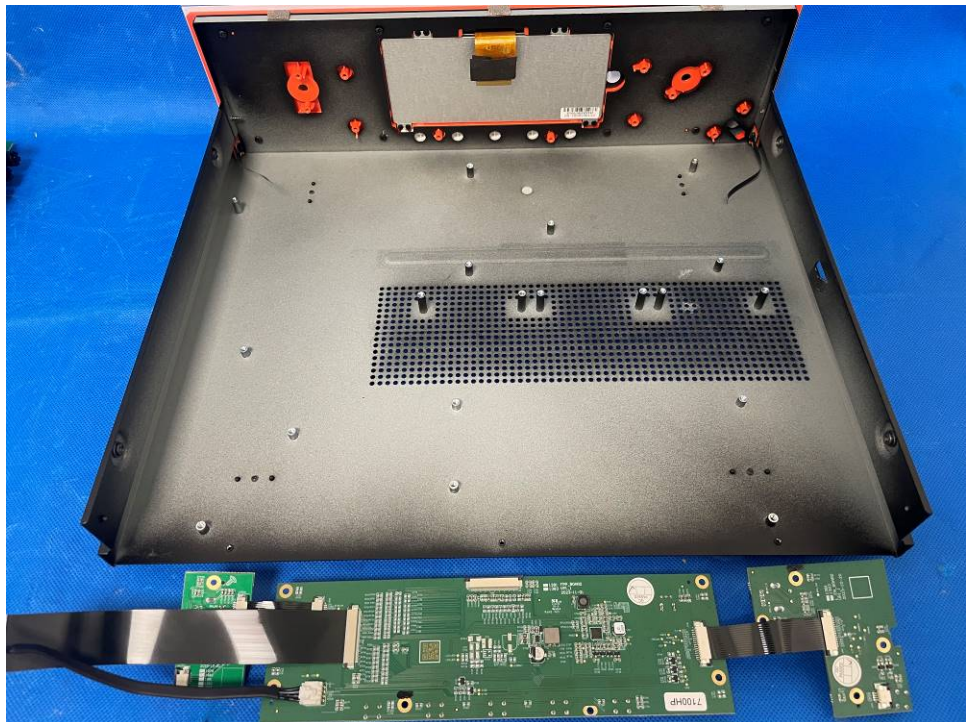
Figure 6. Internal view 6
