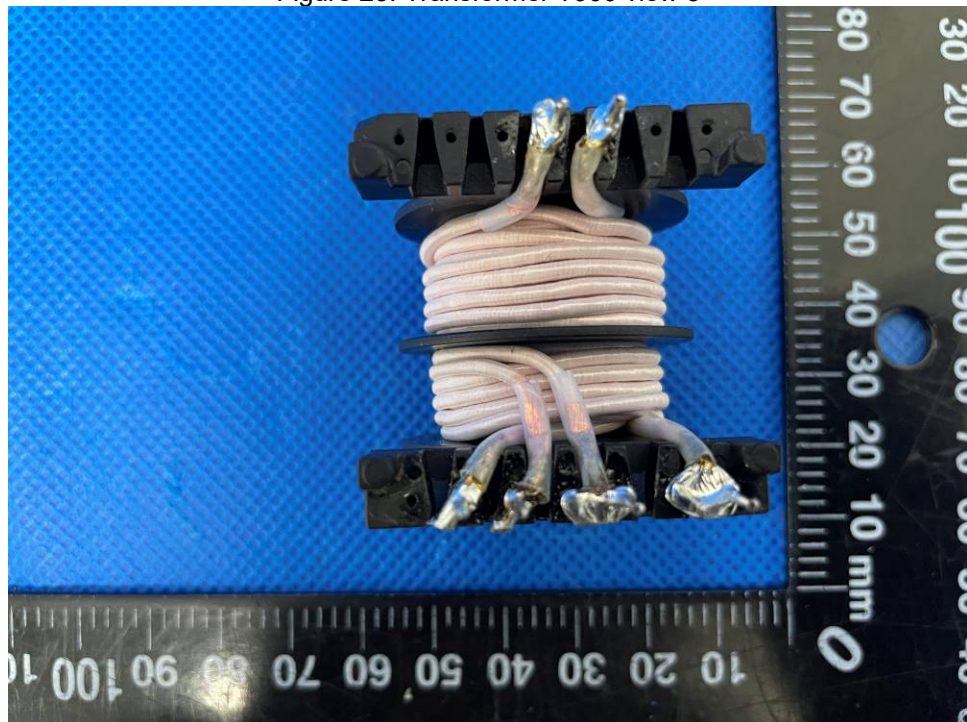
Figure 26. Transformer T900 view 4
