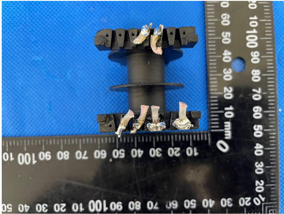
Figure 27. Transformer T900 view 5
