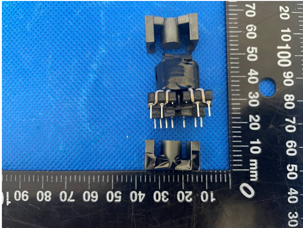
Figure 33. Transformer T901 view 6
