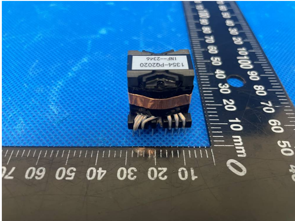
Figure 31. Transformer T901 view 4
