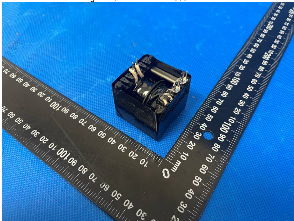
Figure 24. Transformer T900 view 2
