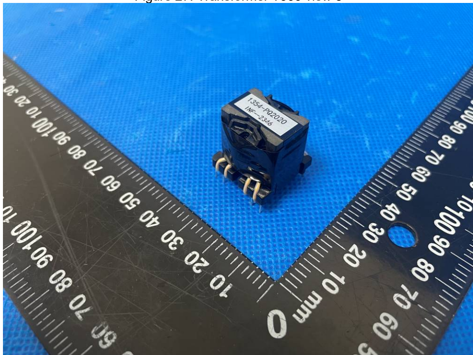
Figure 28. Transformer T901 view 1
