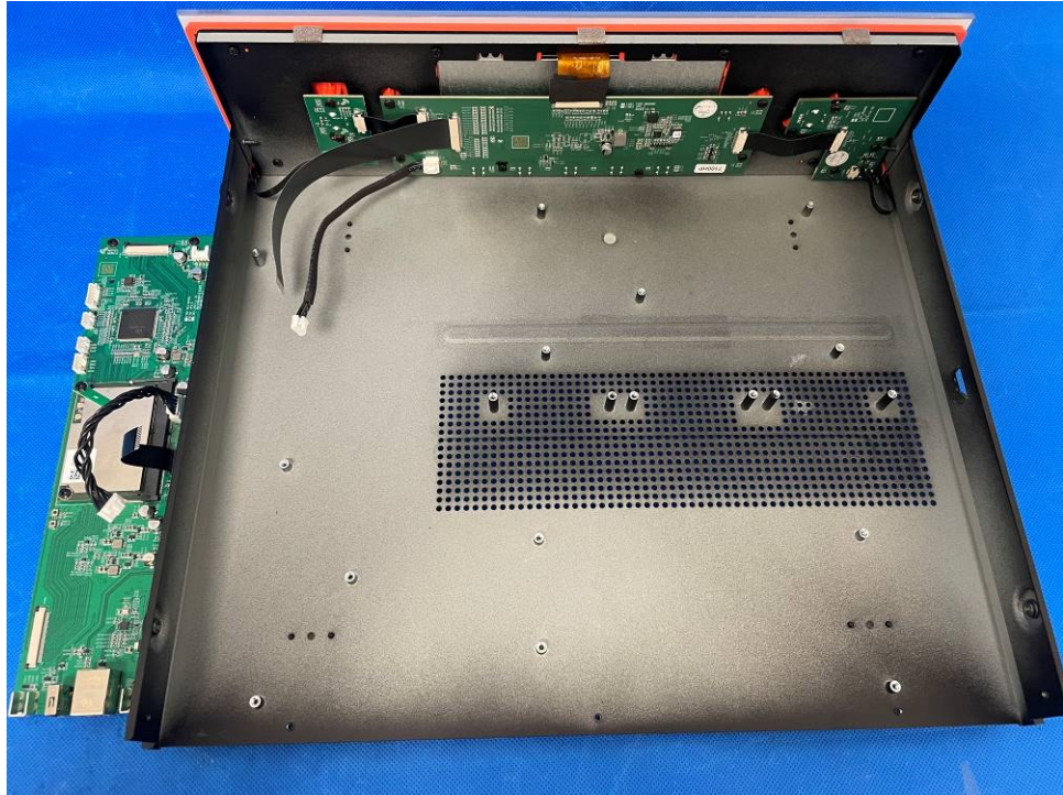
Figure 5. Internal view 5
