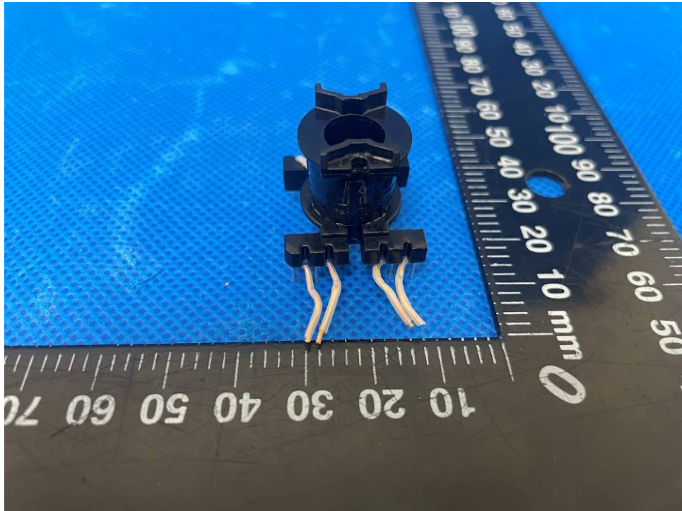
Figure 39. Transformer T901 view 12
