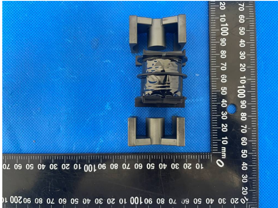
Figure 25. Transformer T900 view 3
