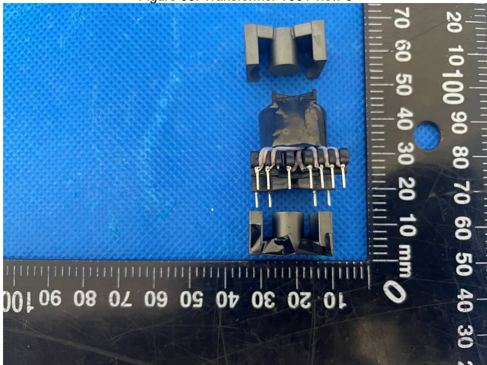
Figure 34. Transformer T901 view 7
