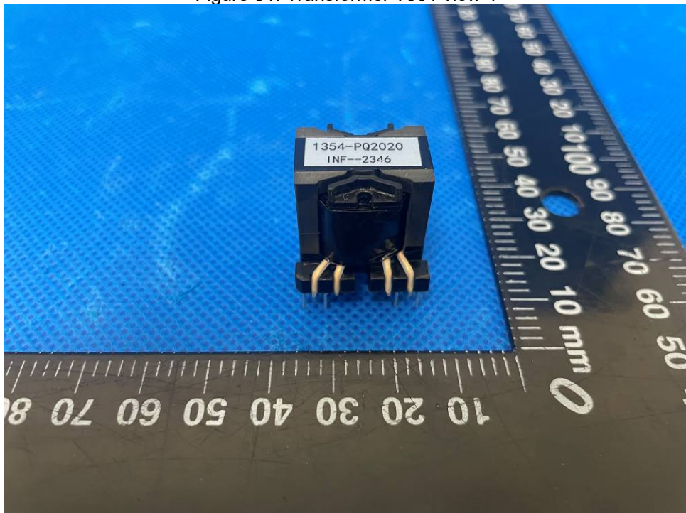
Figure 32. Transformer T901 view 5
