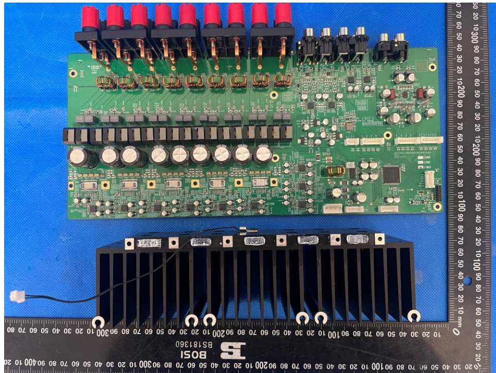
Figure 11. AMP board view 1
