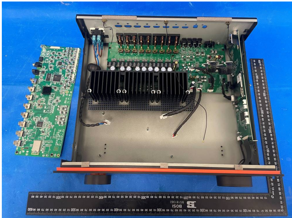
Figure 2. Internal view 2
