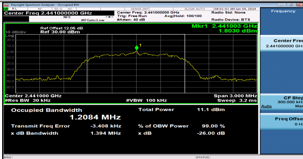
3DH5-Ant1-2441
