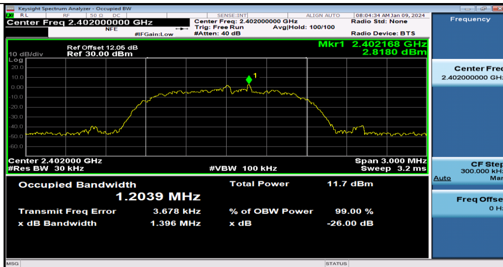
3DH5-Ant1-2402
