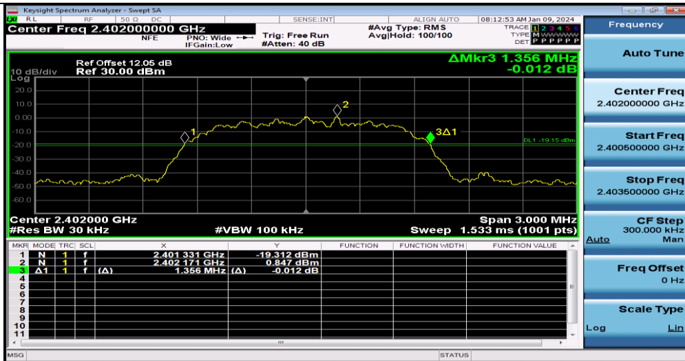
2DH5-Ant1-2402
