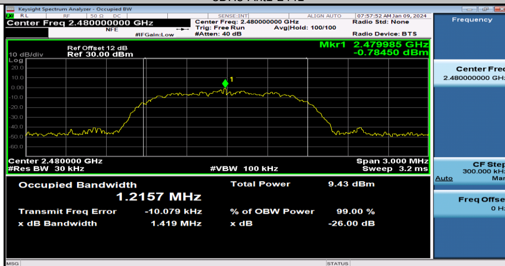
3DH5-Ant1-2480
