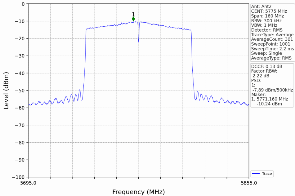
802.11ac(VHT80)_MCH_5775MHz_MIMO_NTNV
