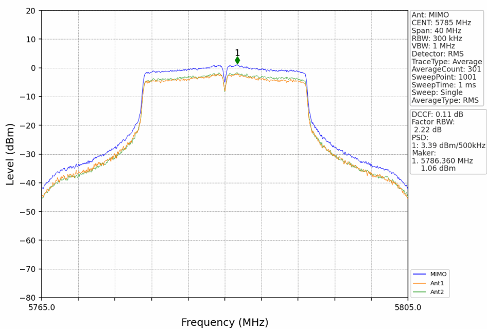
802.11ac(VHT20)_MCH_5785MHz_MIMO_NTNV
