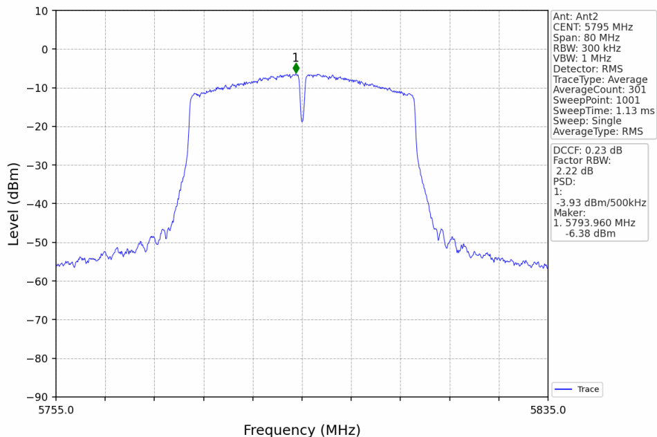
802.11ac(VHT40)_HCH_5795MHz_Ant2_NTNV
