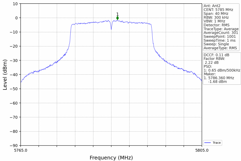
802.11ac(VHT20)_MCH_5785MHz_MIMO_NTNV
