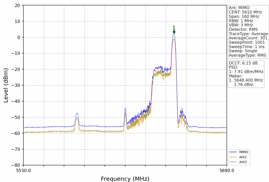
802.11ax(HEW80)_HCH_5610MHz_RU26_Right_MIMO_NTNV
