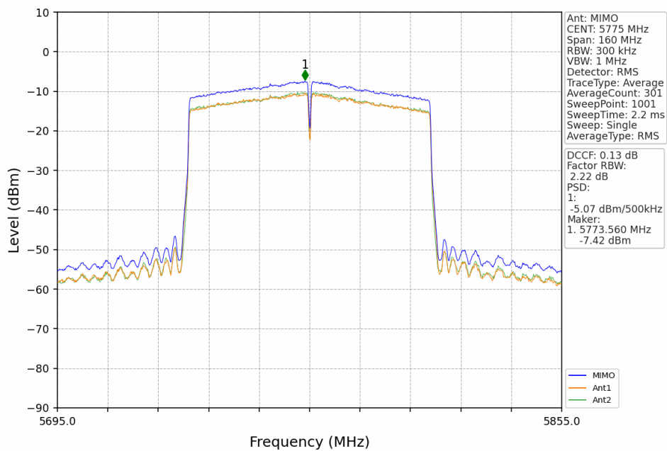
802.11ac(VHT80)_MCH_5775MHz_MIMO_NTNV
