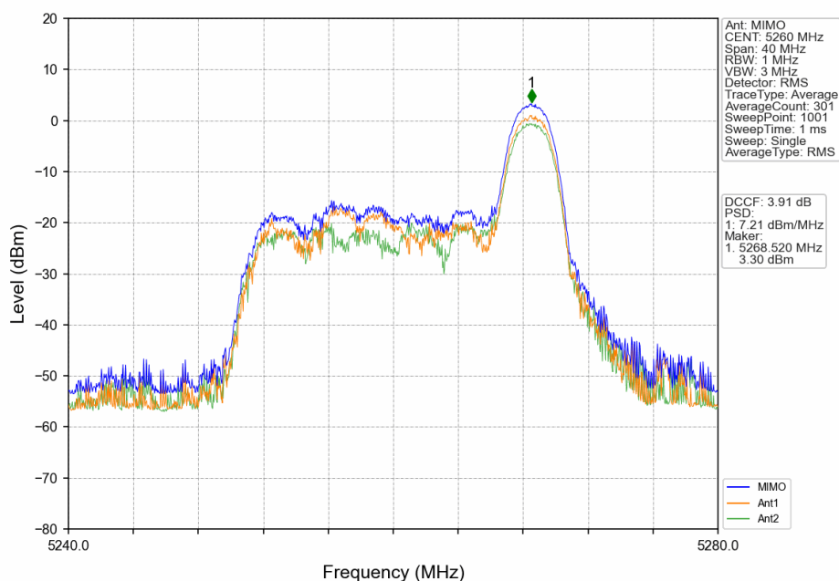
802.11ax(HEW20)_LCH_5260MHz_RU26_Right_MIMO_NTNV
