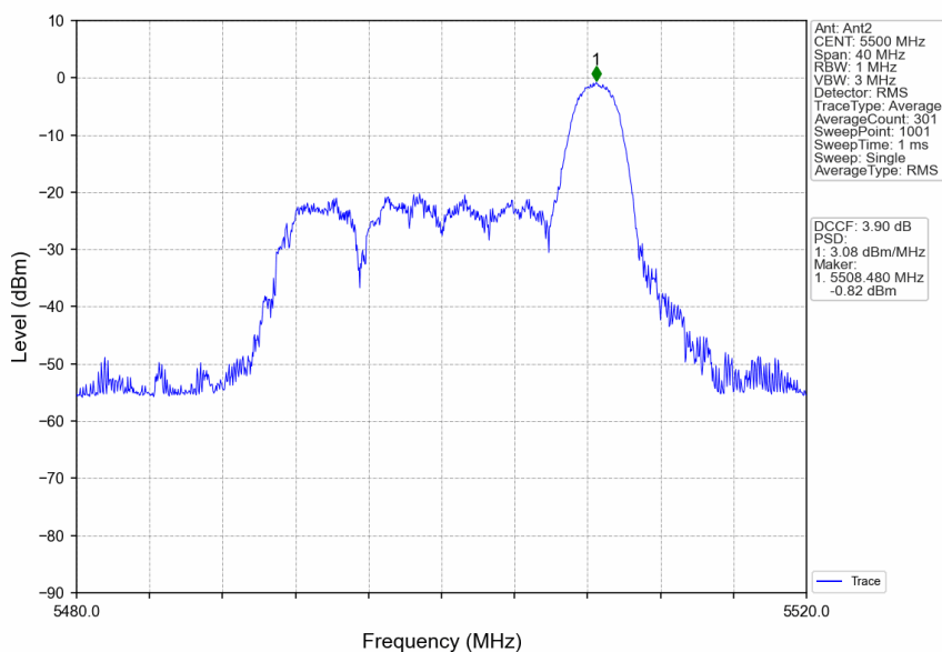
802.11ax(HEW20)_LCH_5500MHz_RU26_Right_MIMO_NTNV
