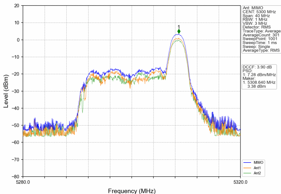
802.11ax(HEW20)_MCH_5300MHz_RU26_Right_MIMO_NTNV
