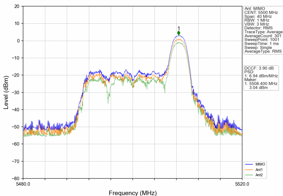
802.11ax(HEW20)_LCH_5500MHz_RU26_Right_MIMO_NTNV
