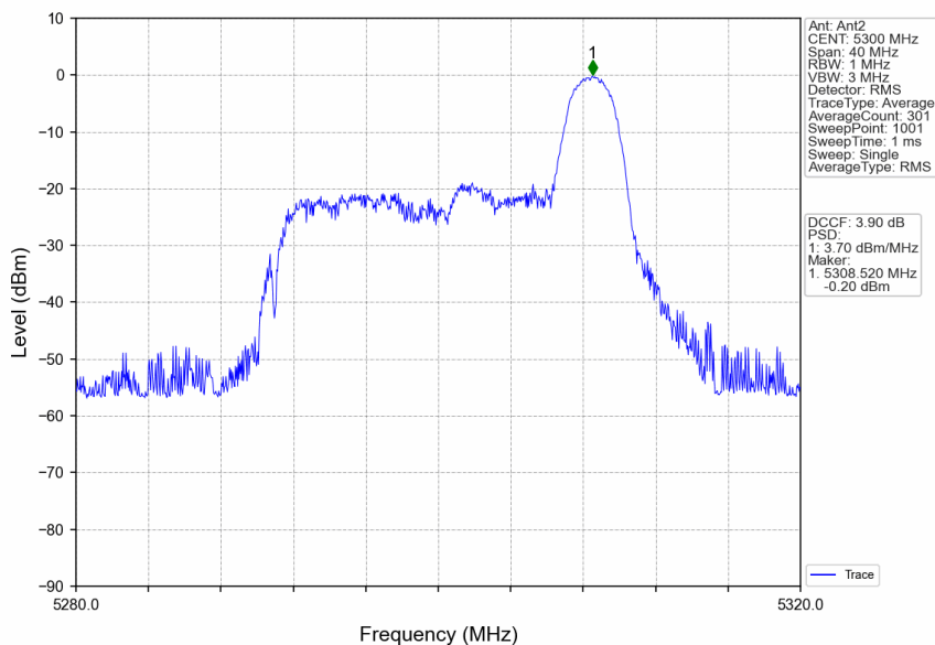
802.11ax(HEW20)_MCH_5300MHz_RU26_Right_MIMO_NTNV
