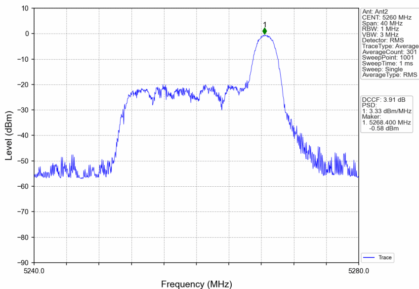
802.11ax(HEW20)_LCH_5260MHz_RU26_Right_MIMO_NTNV
