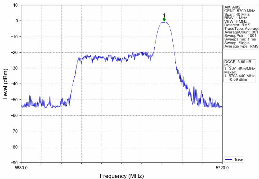
802.11ax(HEW20)_HCH_5700MHz_RU26_Right_MIMO_NTNV
