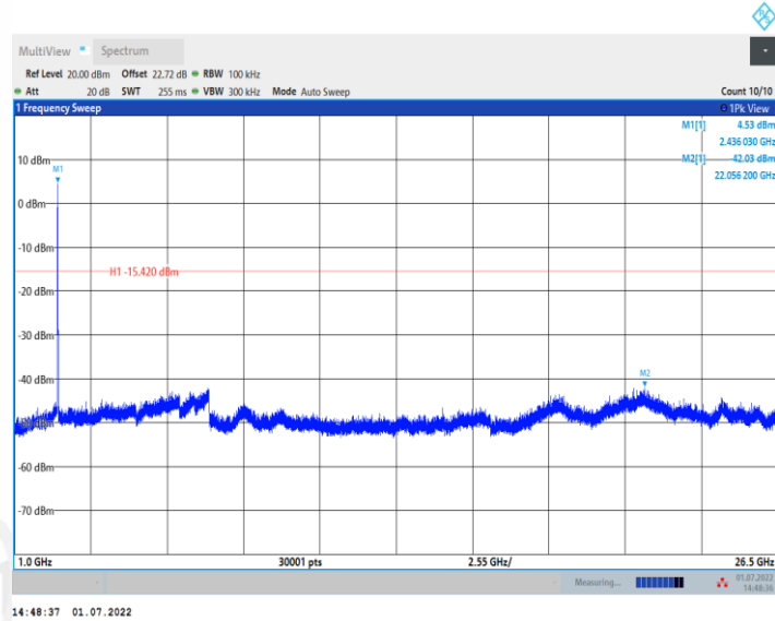
11G_Ant2_2437_0~Reference
