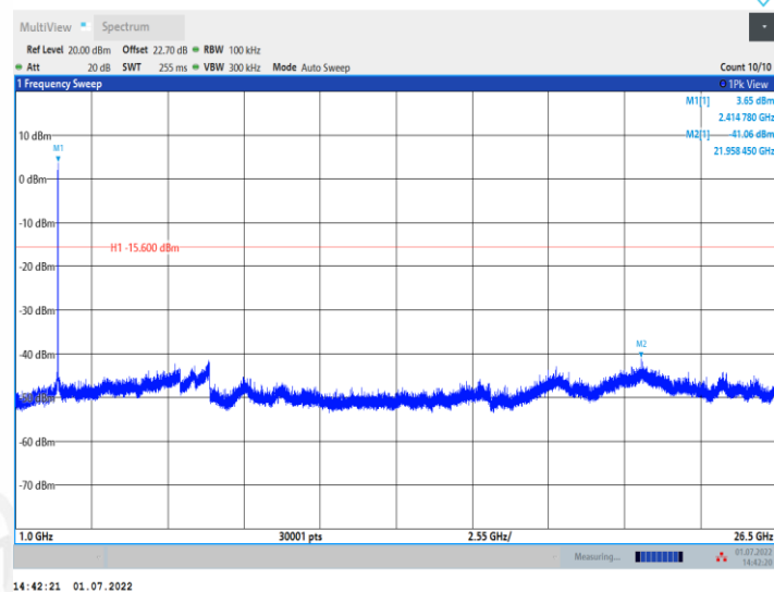
11G_Ant2_2412_0~Reference
