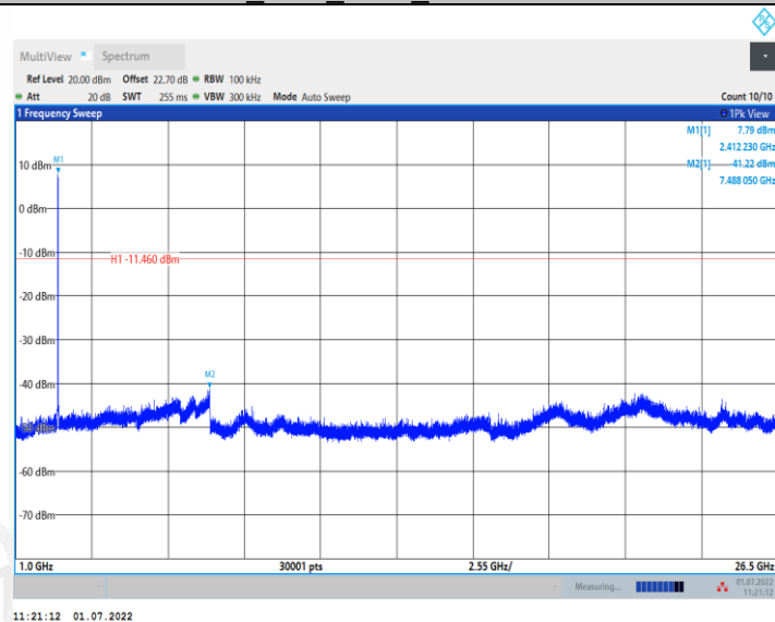
11B_Ant2_2412_0~Reference
