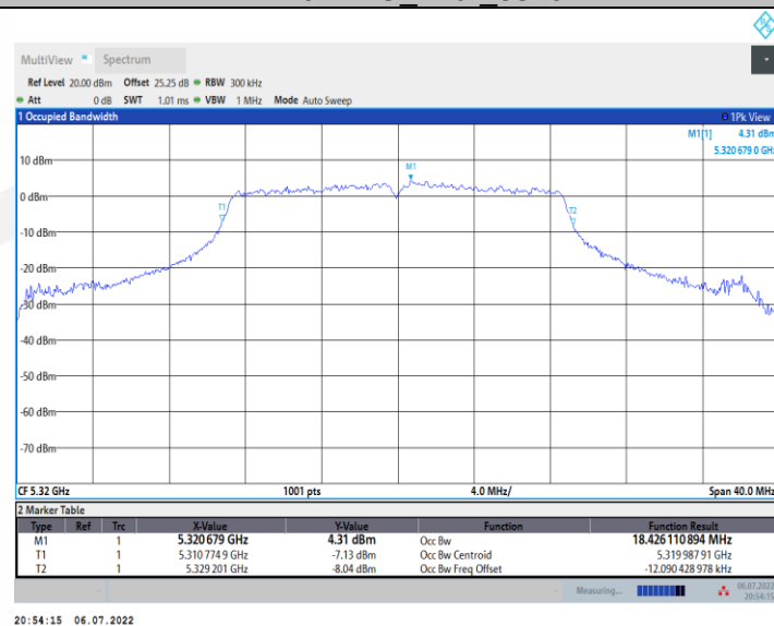
11N20MIMO Ant2 5320
