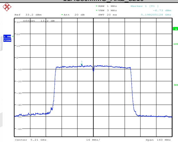
11AC80MIMO Ant2 5210
