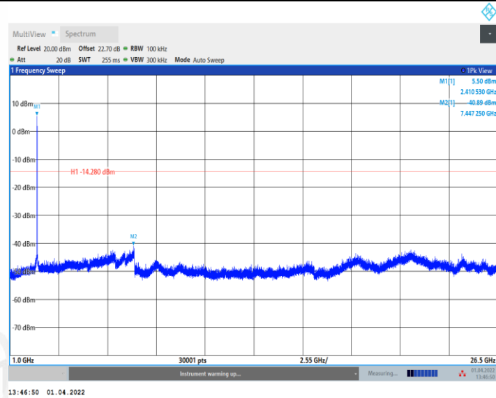
11G_Ant2_2412_0~Reference
