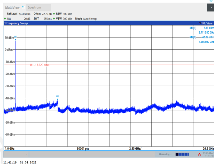
11B_Ant2_2412_0~Reference
