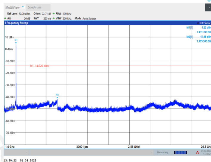
11G_Ant2_2437_0~Reference
