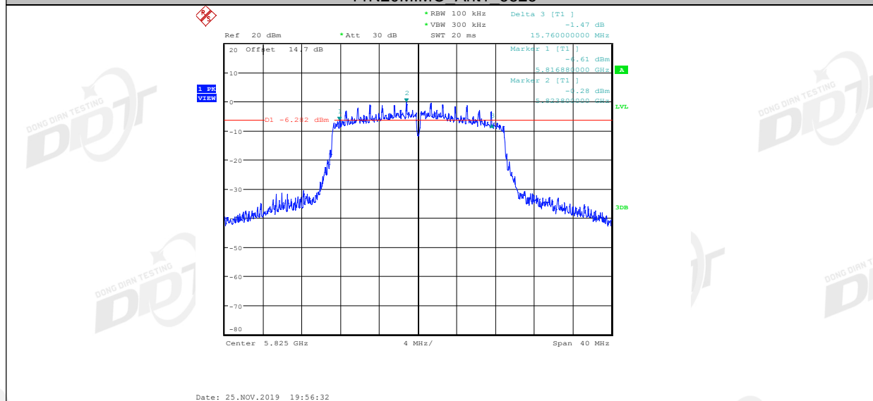
11N20MIMO Ant2 5825
