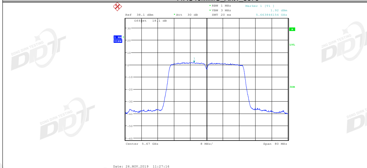
11AC40MIMO Ant2 5670
