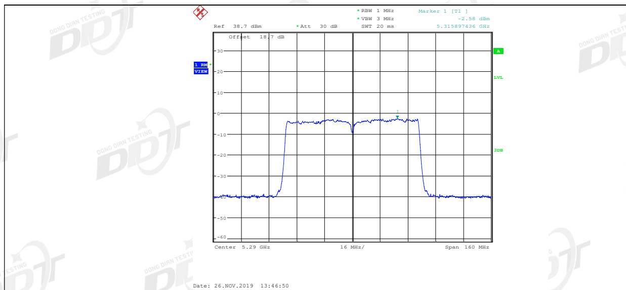
11AC80MIMO Ant2 5290
