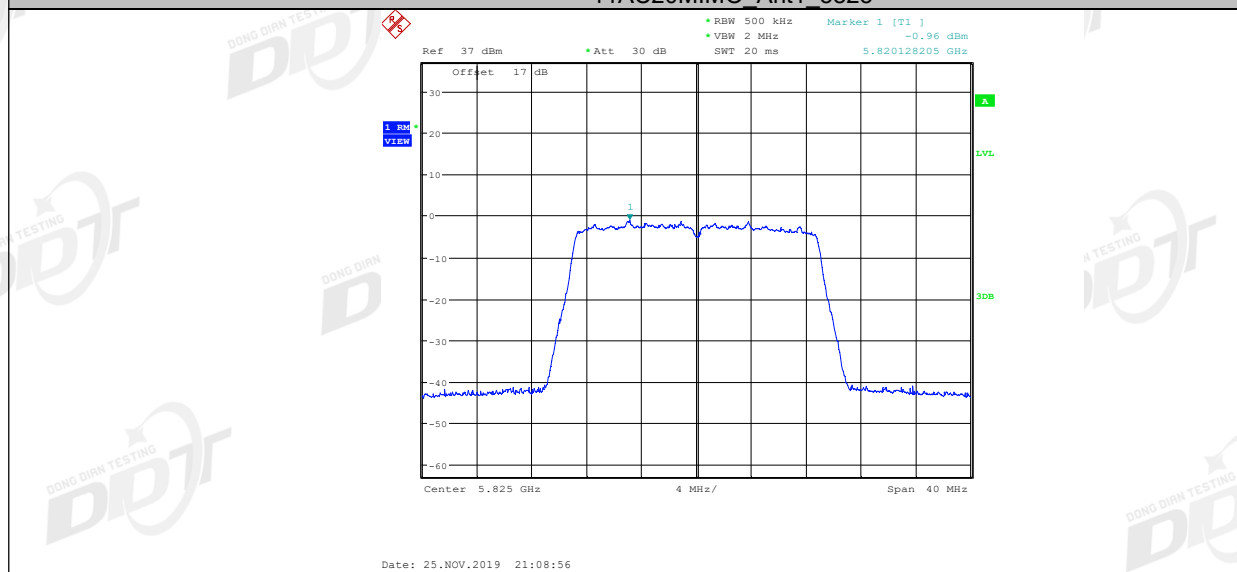
11AC20MIMO Ant2 5825
