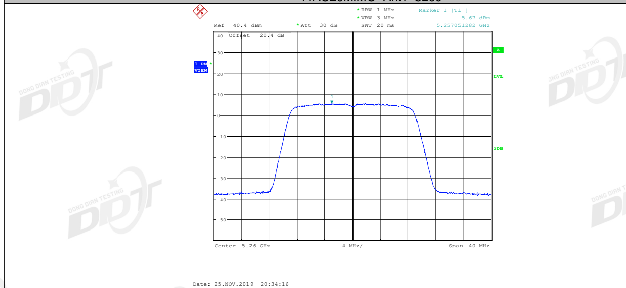
11AC20MIMO Ant2 5260
