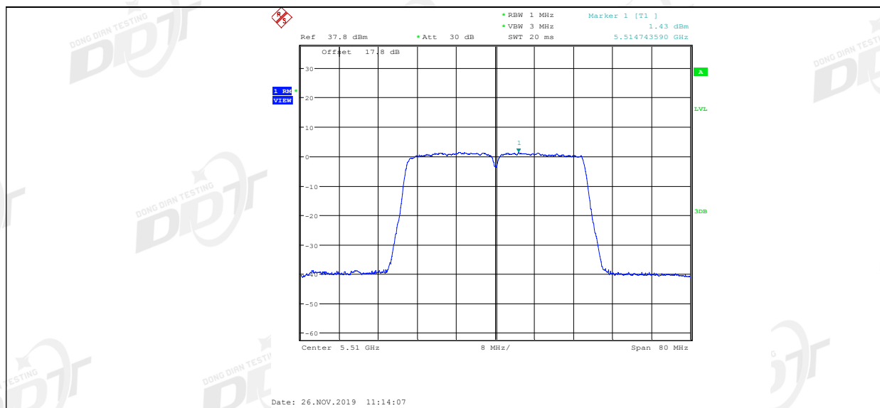
11AC40MIMO Ant2 5510
