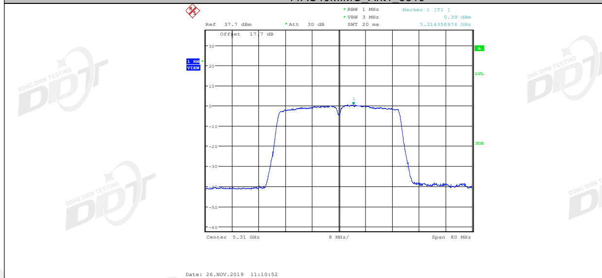
11AC40MIMO Ant2 5310
