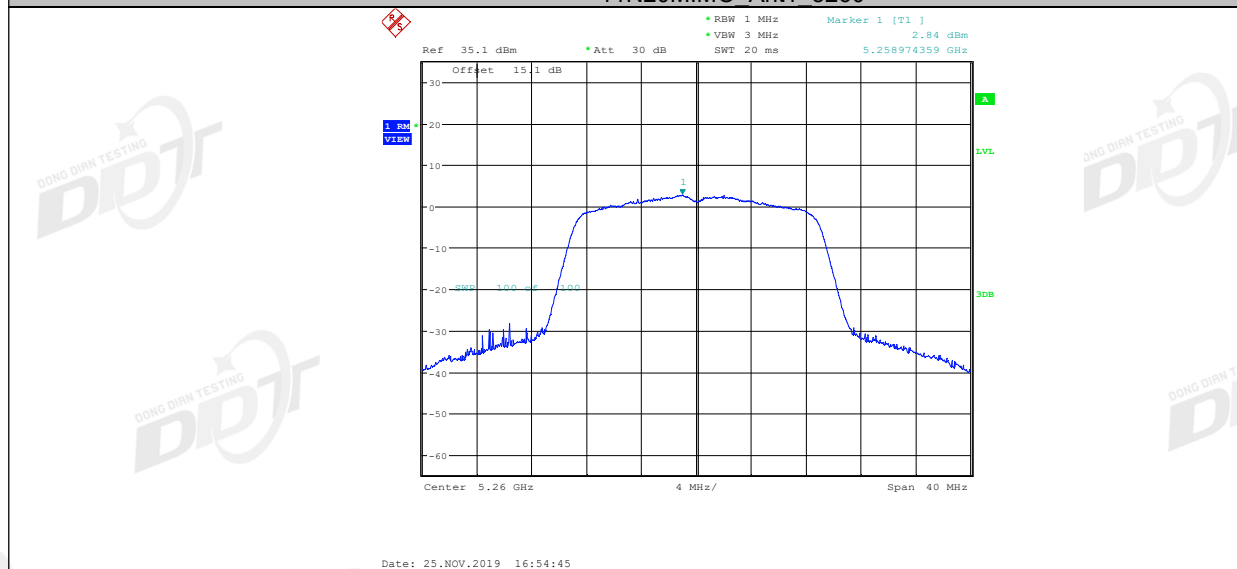
11N20MIMO Ant2 5260
