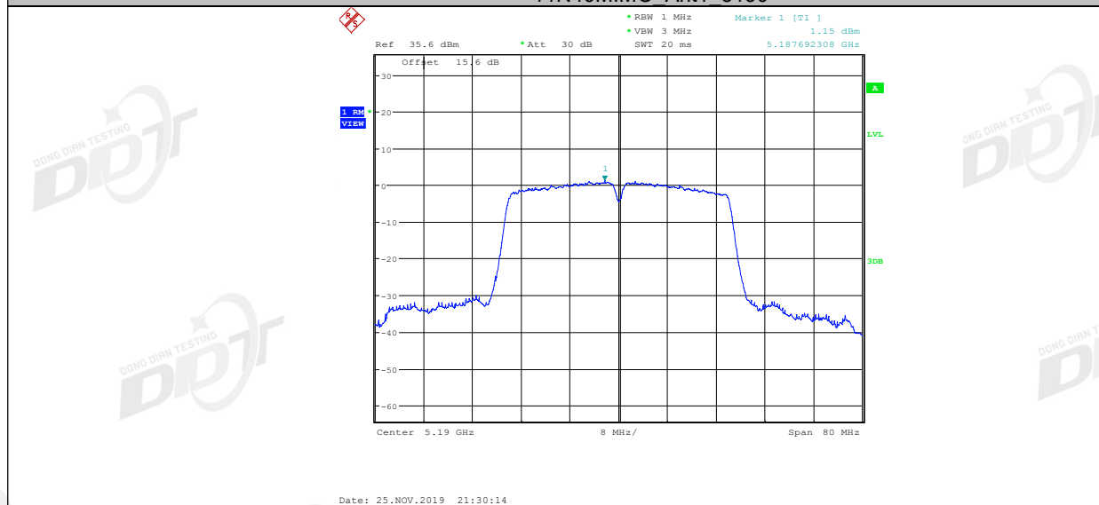
11N40MIMO Ant2 5190
