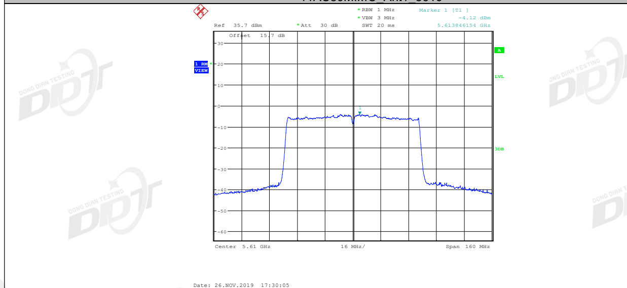
11AC80MIMO Ant2 5610
