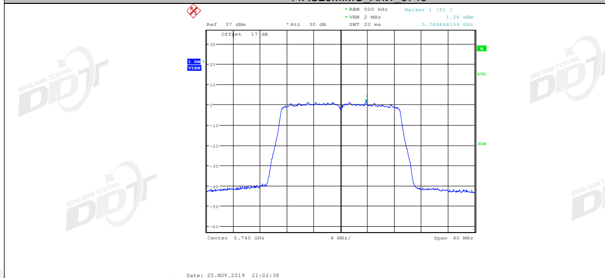
11AC20MIMO Ant2 5745
