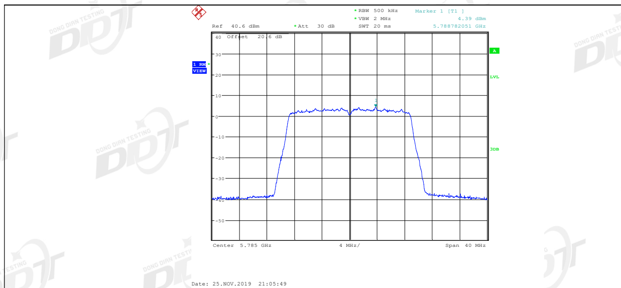
11AC20MIMO Ant2 5785
