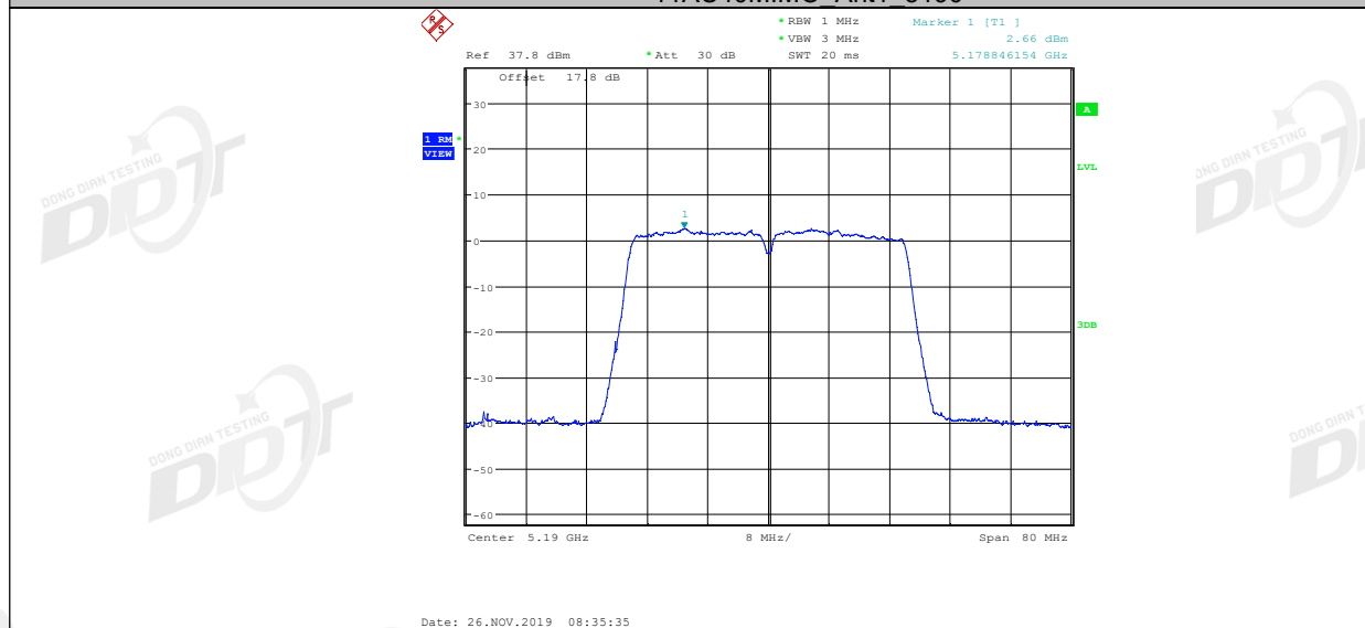
11AC40MIMO Ant2 5190
