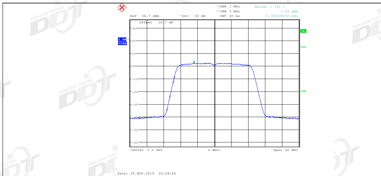
11AC20MIMO Ant2 5200
