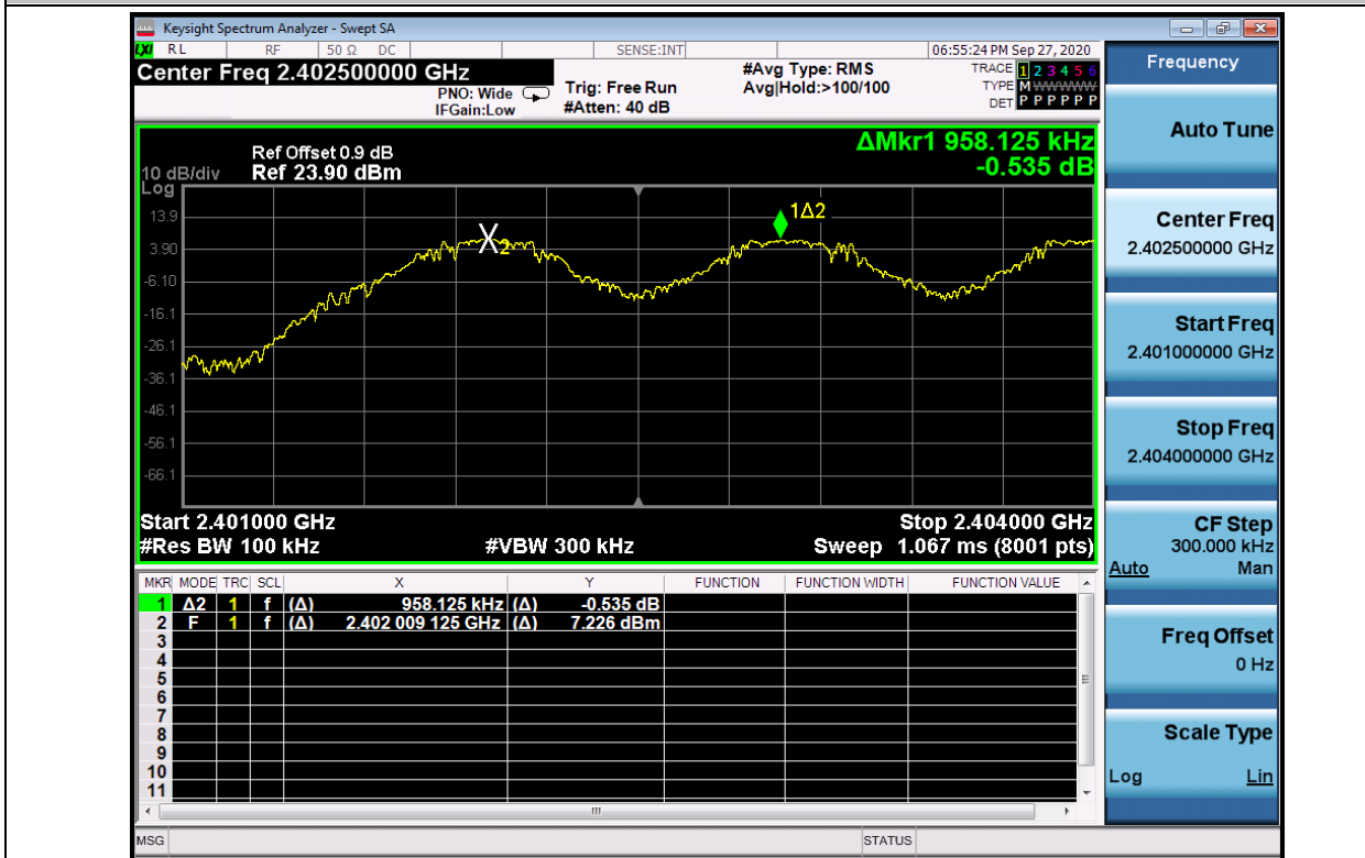
Carrier Frequency Separation_DH5_2402
