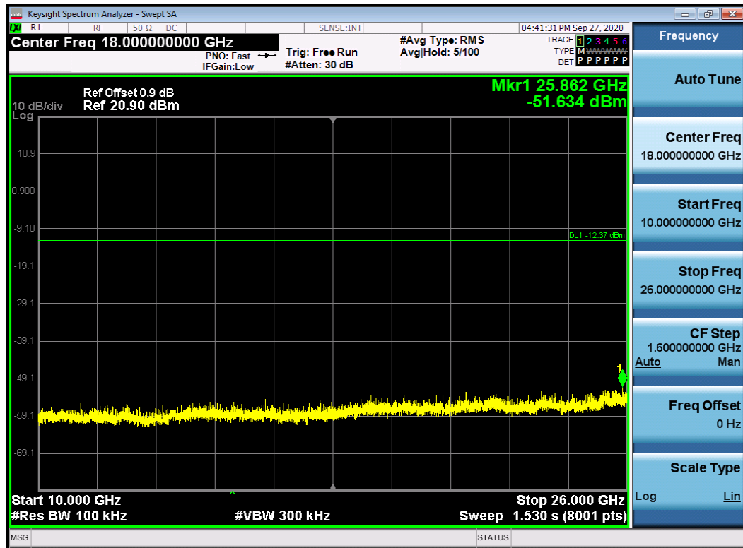
RF Conducted Spurious Emissions_2DH5_2402
