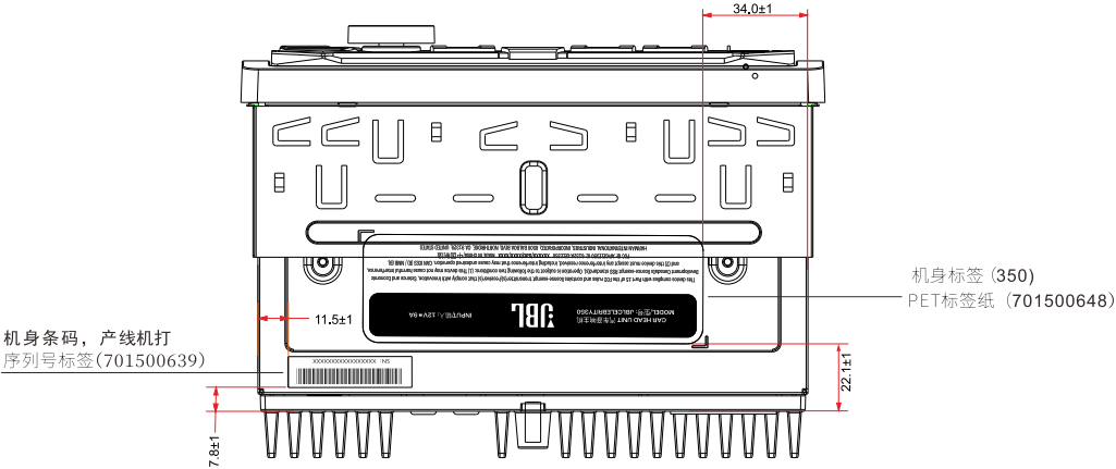
Label position/标签粘贴
