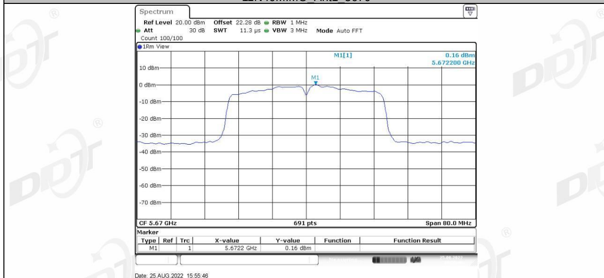
11N40MIMO Ant2 5670
