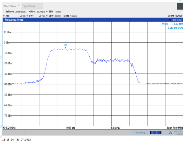
11AX20MIMO Ant2_5260_106Tone_RU54
