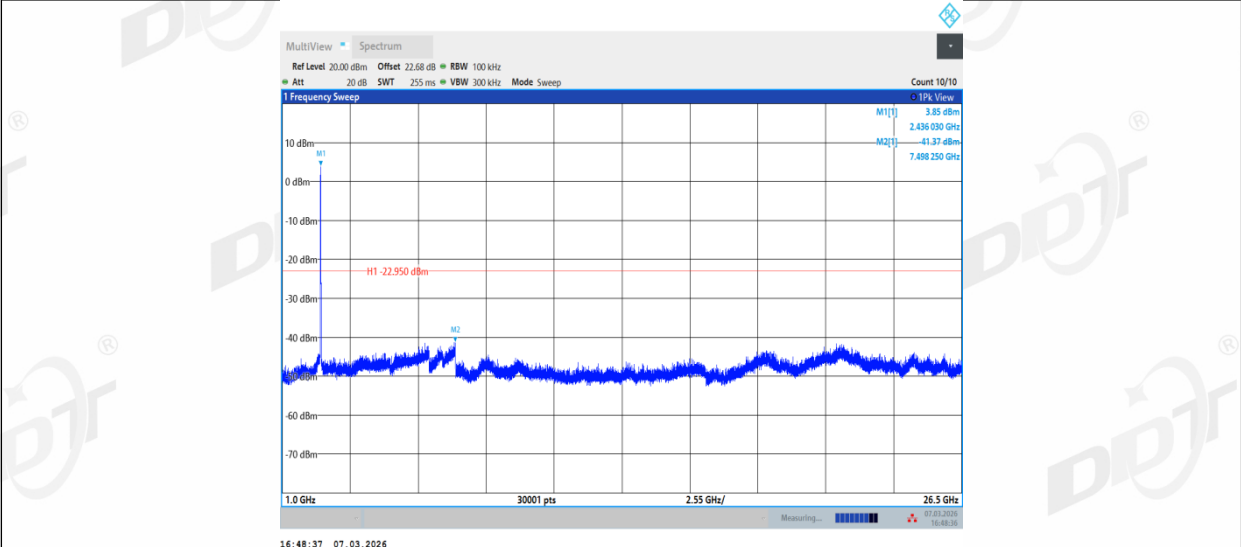
11G_Ant2_2437_0~Reference
