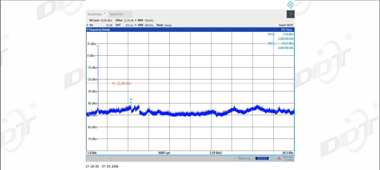
11G_Ant1_2462_0~Reference
