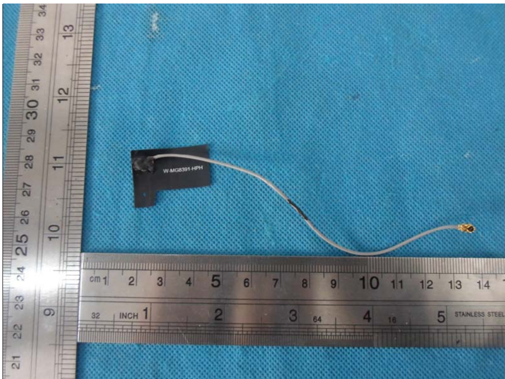
Photo 12 BT Antenna
