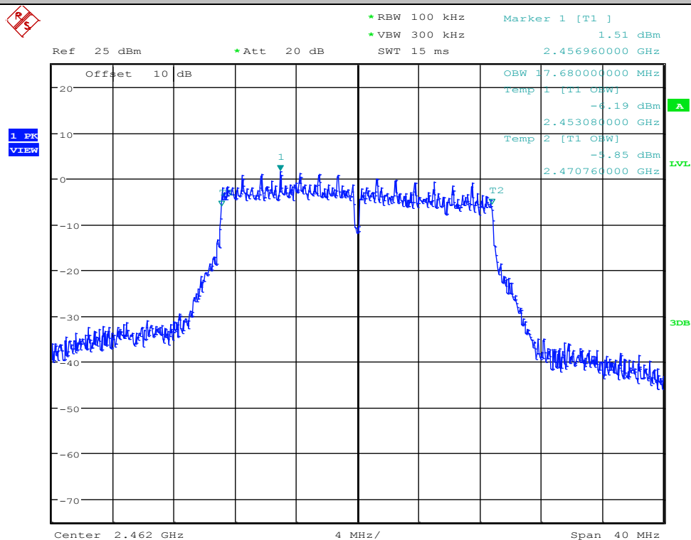
Occupied Bandwidth_11N20MIMO_2462_Ant2
