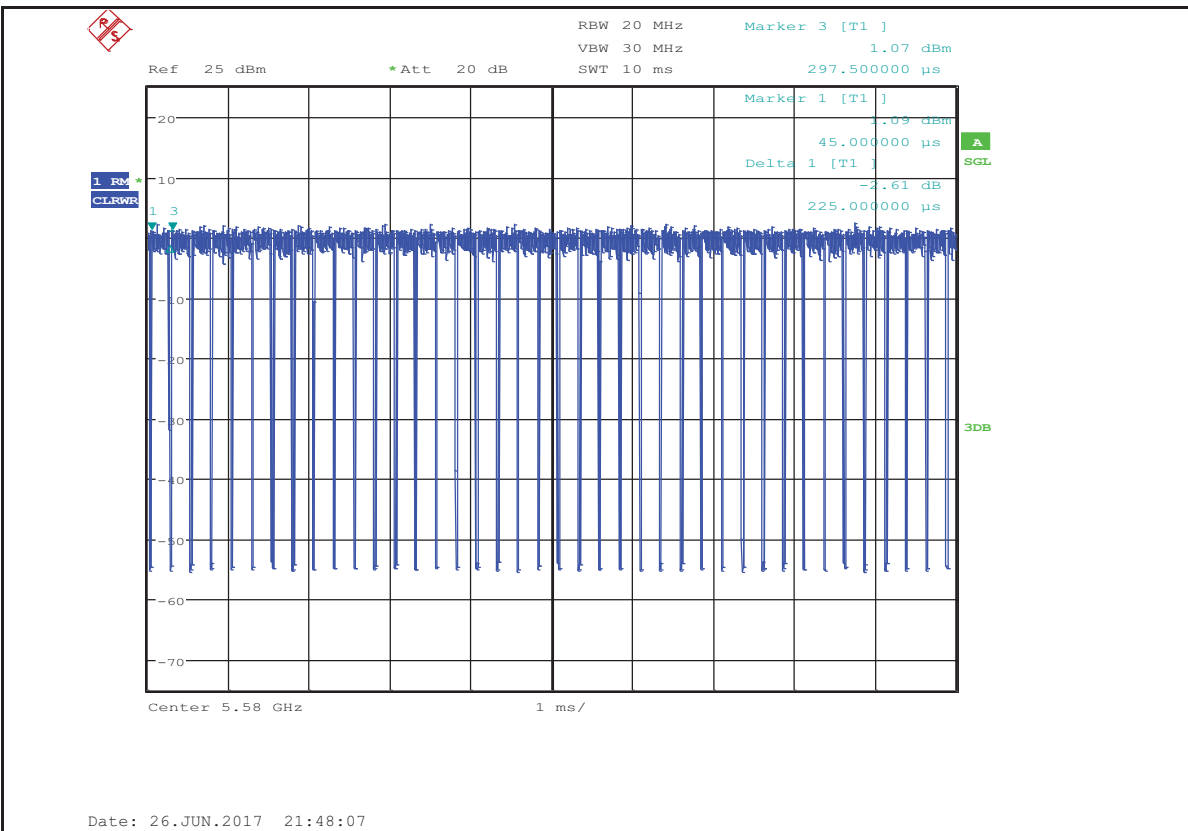
Duty Cycle_11N20MIMO_5580_Ant2
