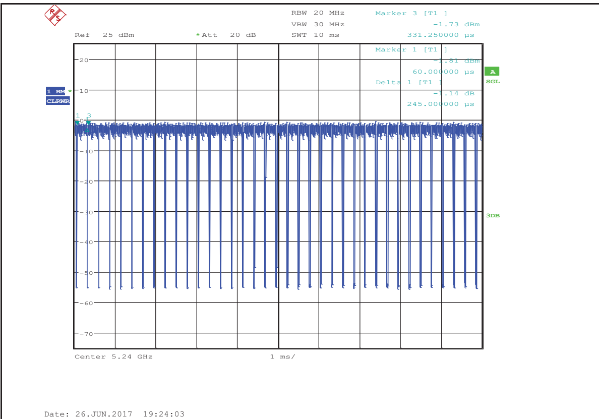
Duty Cycle_11AMIMO_5240_Ant2
