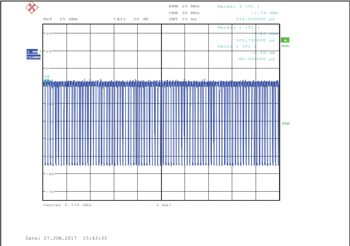
Duty Cycle_11AC80MIMO_5775_Ant2
