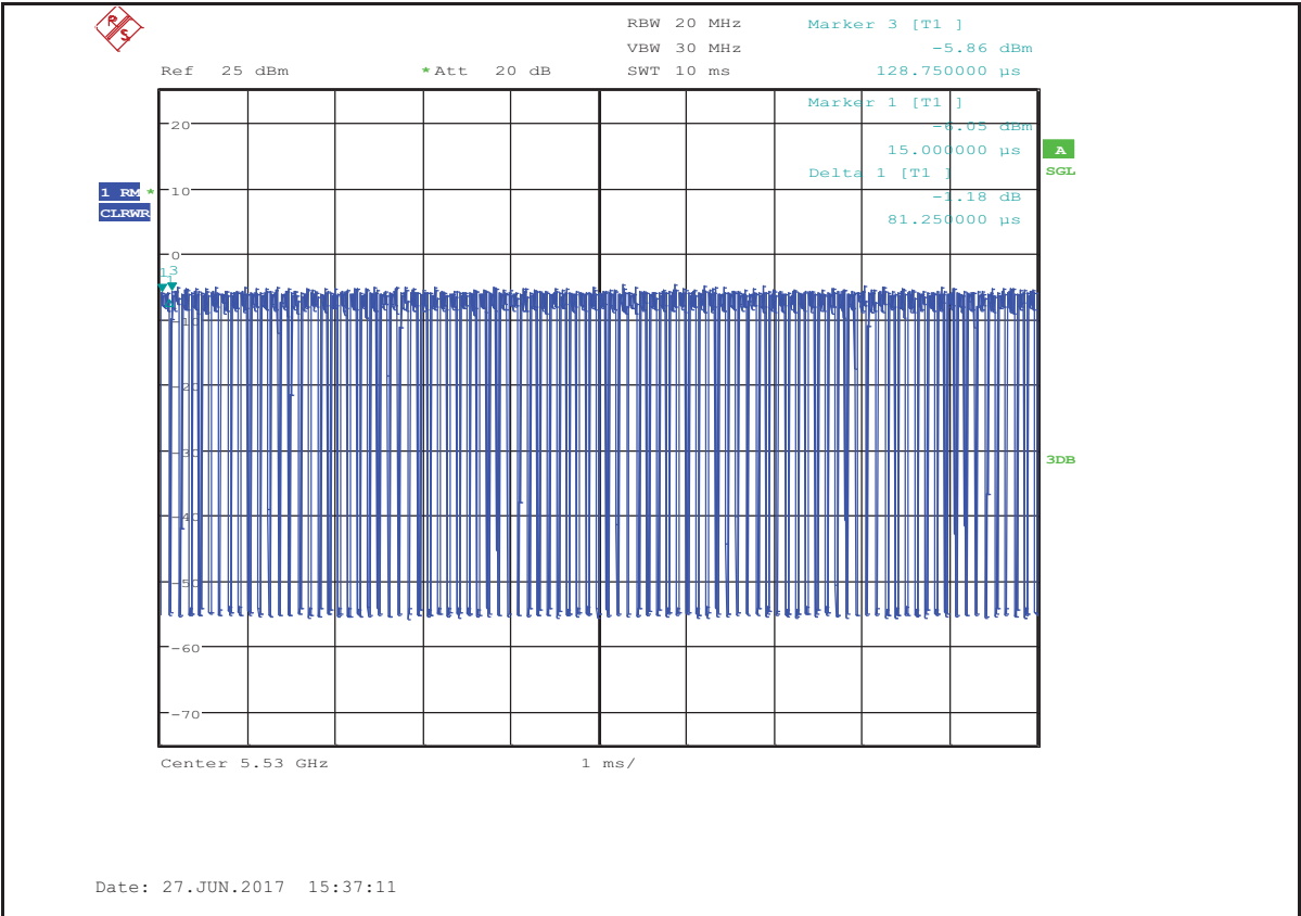
Duty Cycle_11AC80MIMO_5530_Ant2
