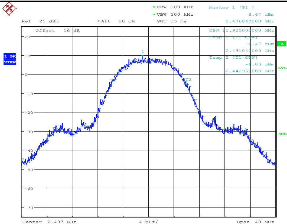
99% Occupied Bandwidth_11B_2437_Ant2
