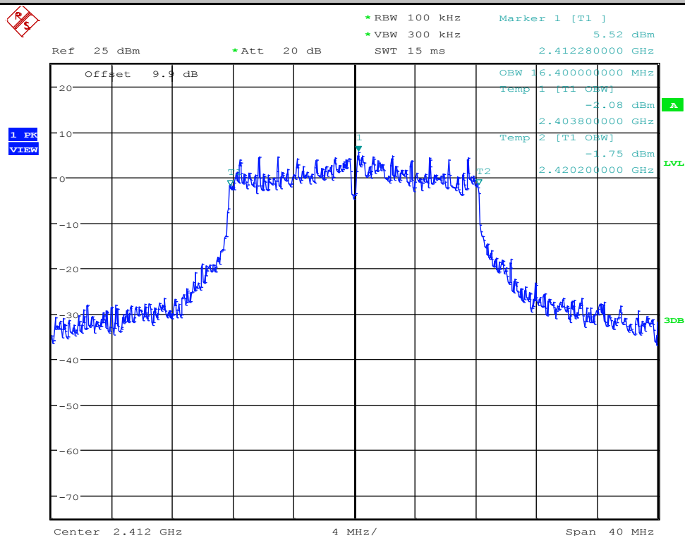
99% Occupied Bandwidth_11G_2412_Ant1
