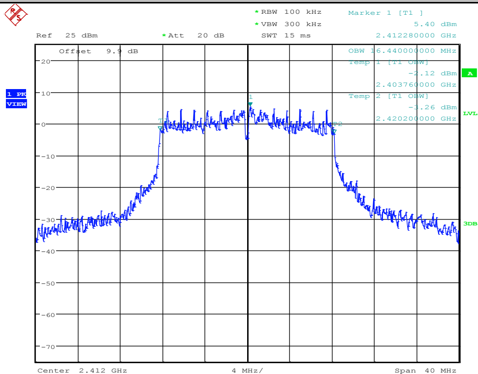
99% Occupied Bandwidth_11G_2412_Ant2
