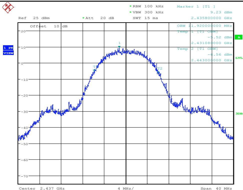
99% Occupied Bandwidth_11B_2437_Ant1
