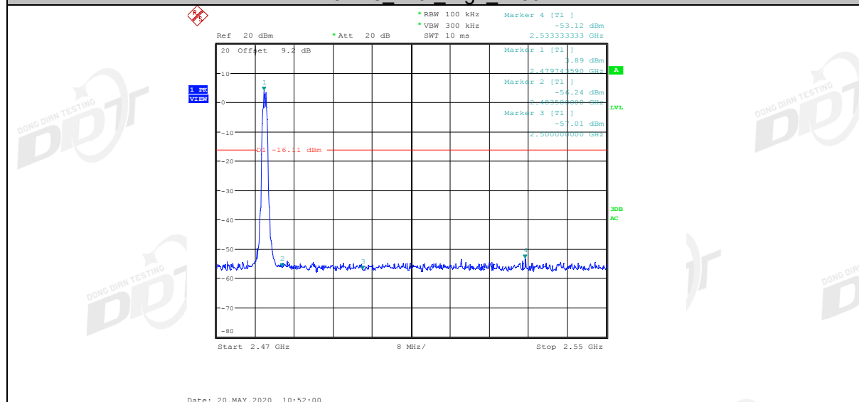
3DH5_Ant2_High_2480
