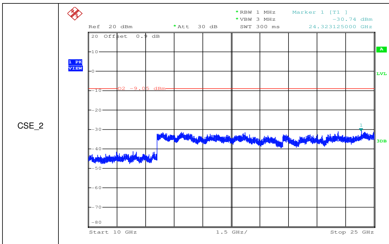
RF Conducted Spurious Emissions_11B_2437_Ant2
