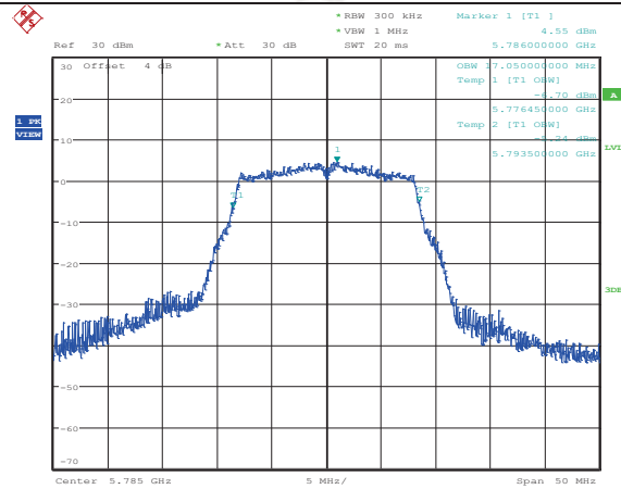
11A_ANT2_5785_99% Bandwidth
