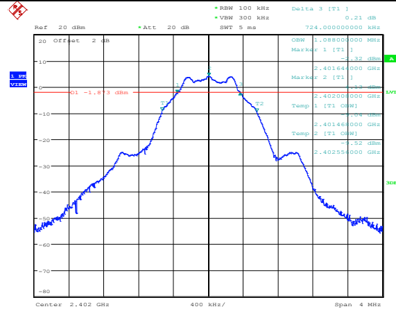
BLE_ANT1_2402_6 dB bandwidth
