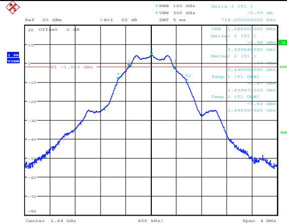
BLE_ANT1_2440_6 dB bandwidth
