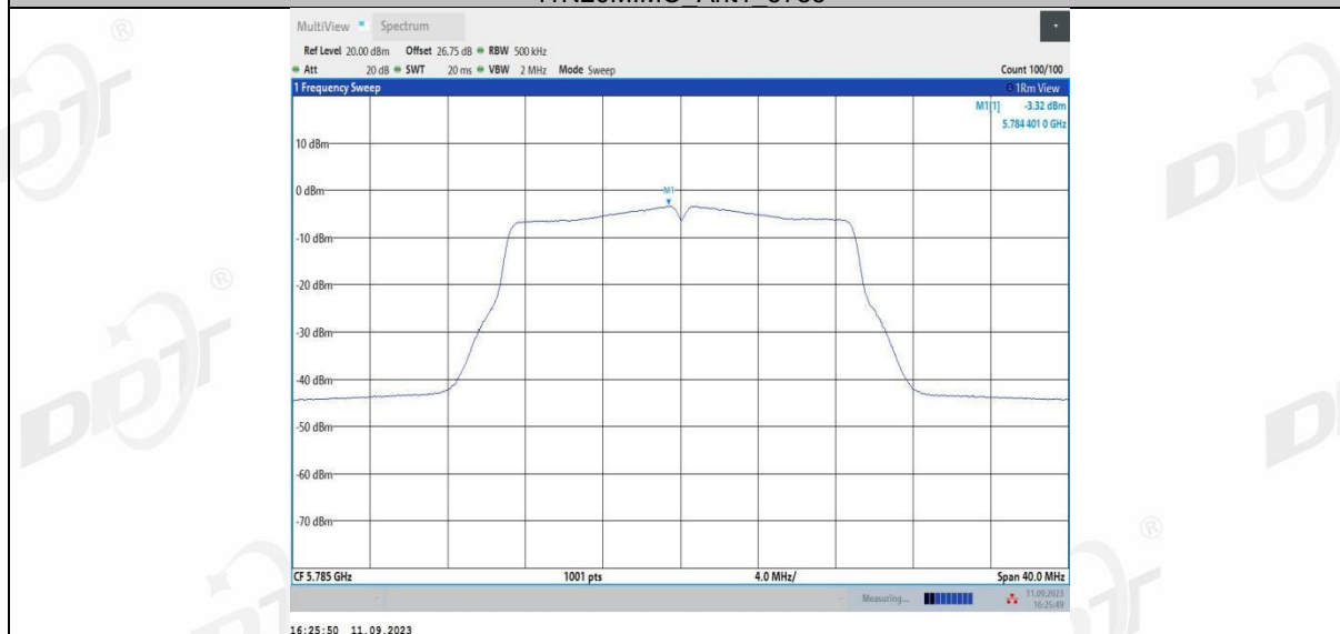
11N20MIMO Ant2 5785
