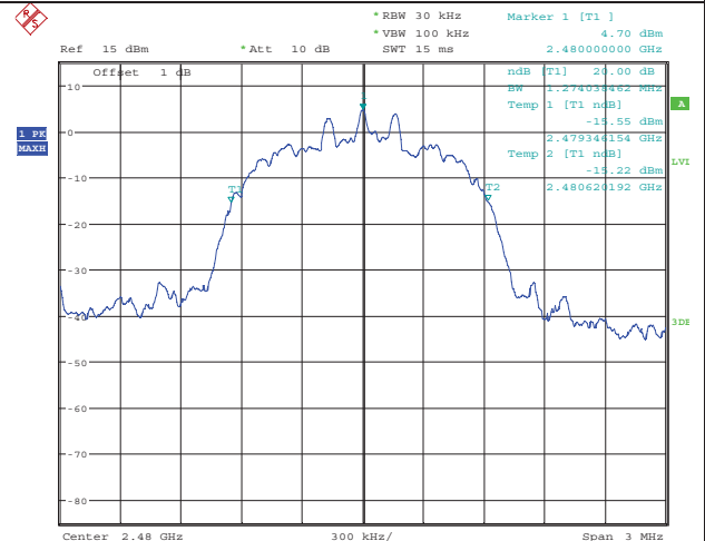
8-DPSK Mode 2480MHz
