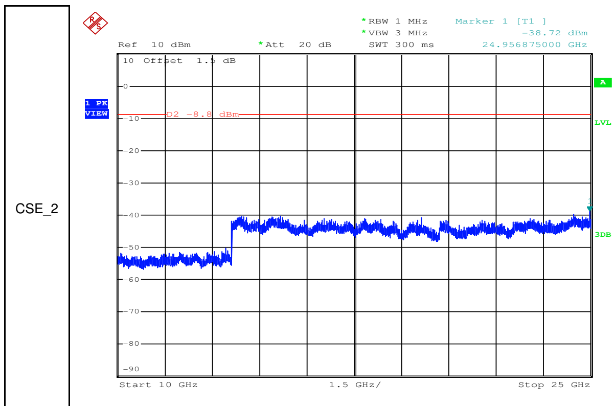
RF Conducted Spurious Emissions_11B_2412_Ant2
