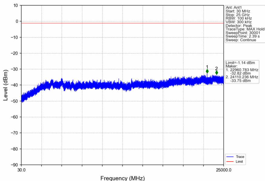
Zigbee_HCH_2475MHz_Ant1_NTNV
