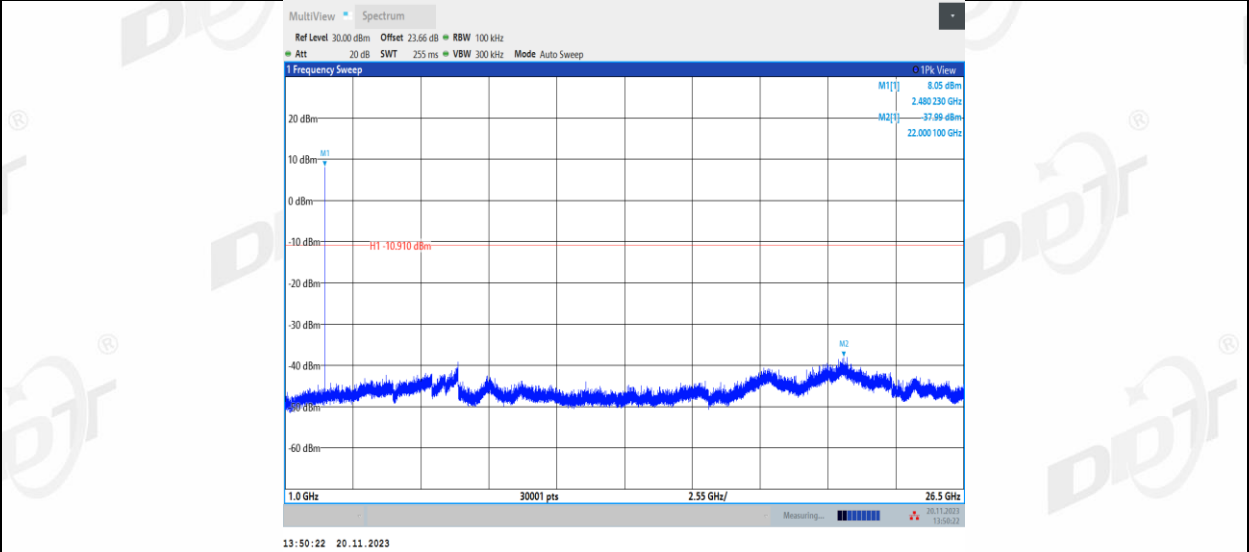
2DH5_Ant1_2402_0~Reference
