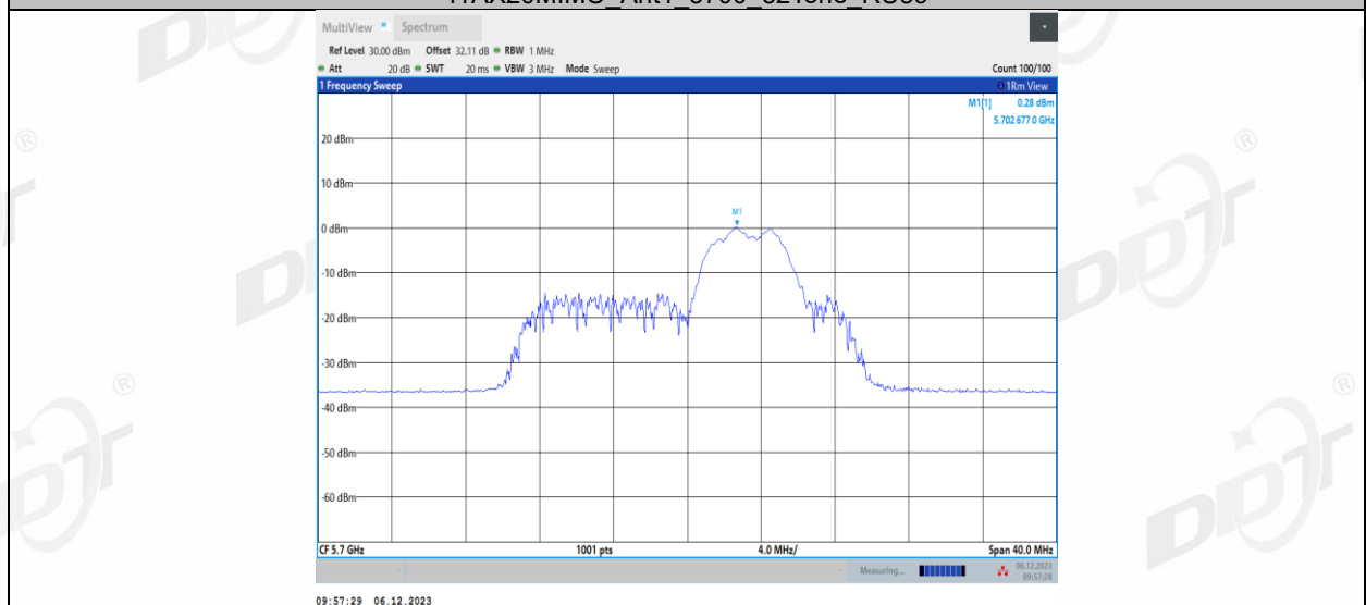
11AX20MIMO Ant1 5700_52Tone_RU40
