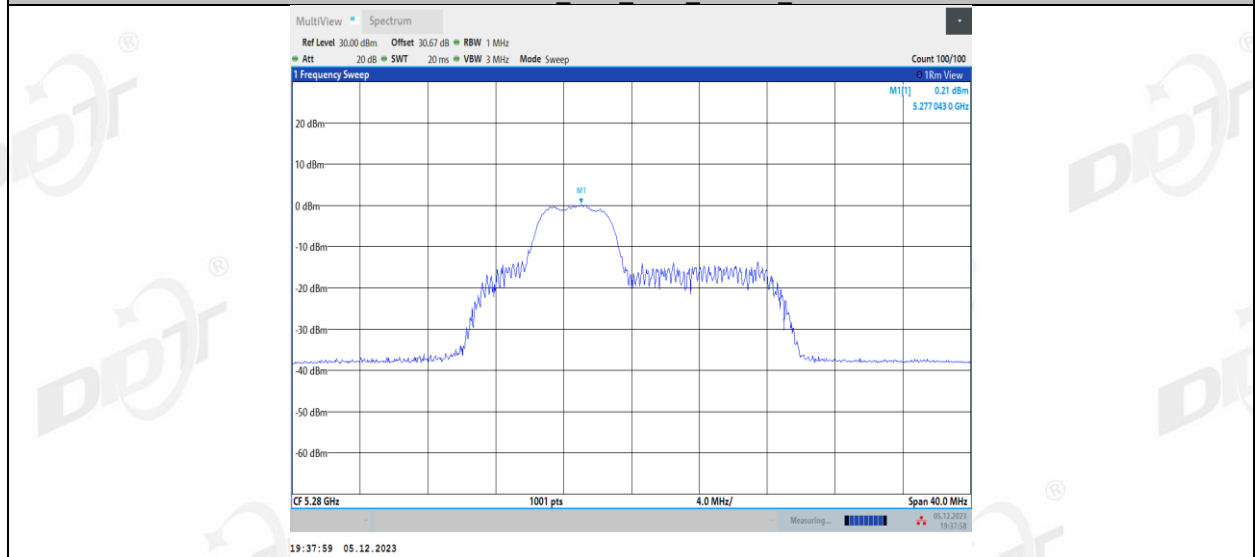
11AX20MIMO Ant2 5280_52Tone_RU39
