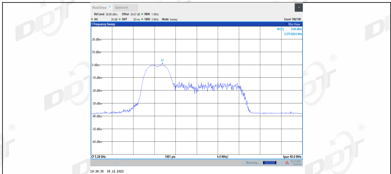
11AX20MIMO Ant2 5280_52Tone_RU38
