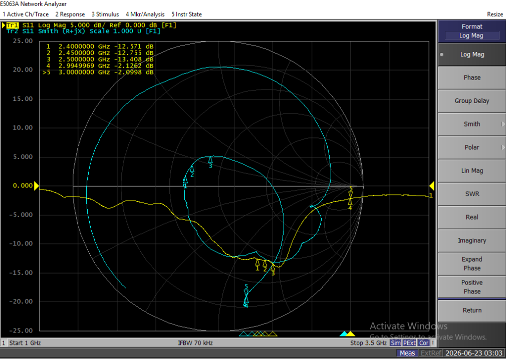
Return loss
