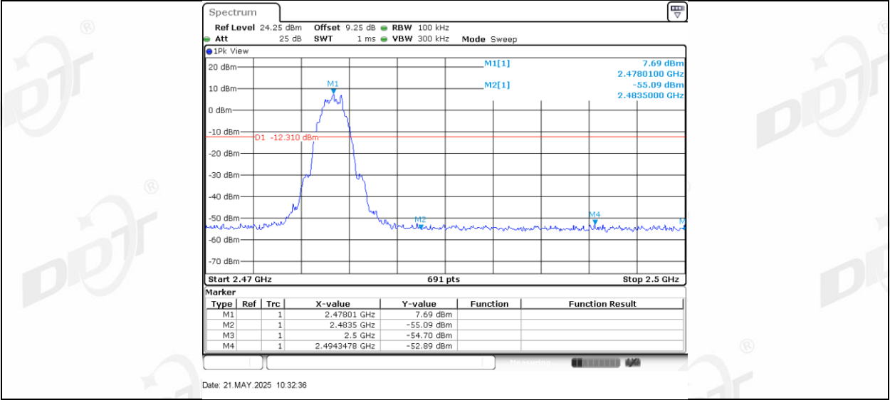
BLE_2M_Right side_High_2478
