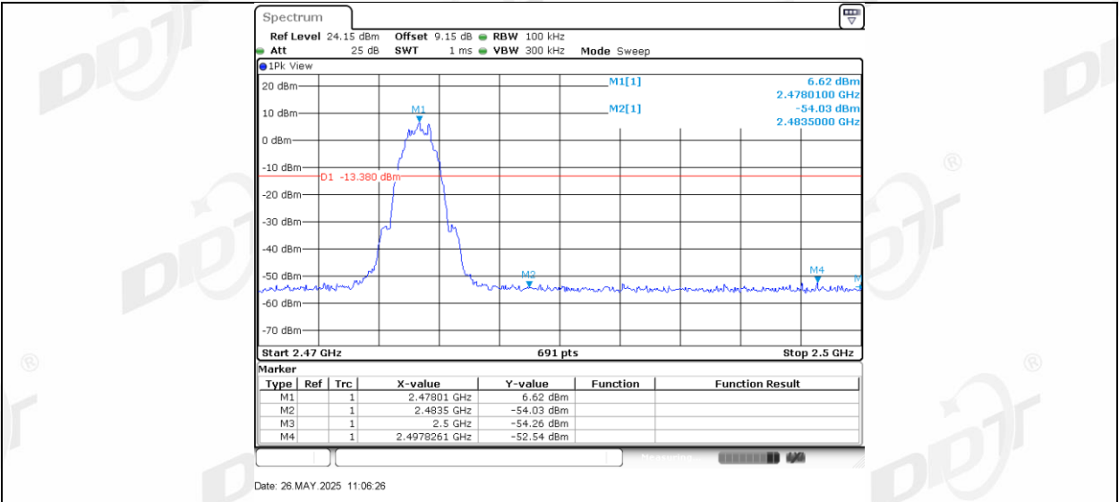
BLE_2M_Right side_High_2478
