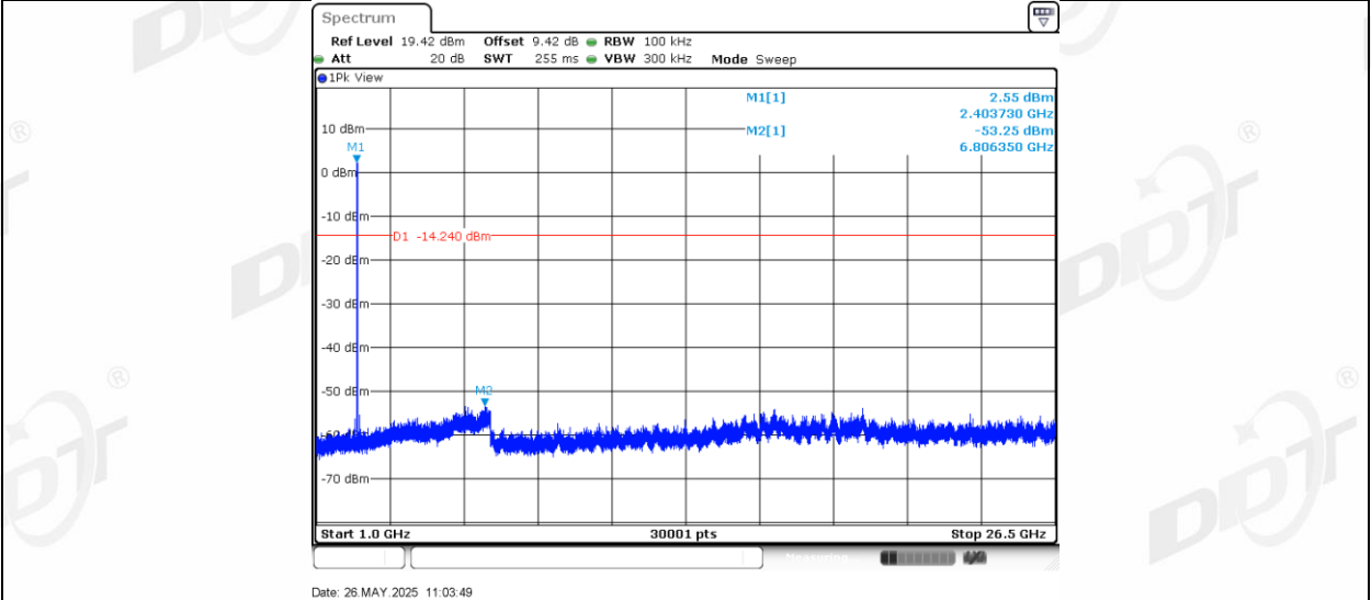
BLE_2M_Right side_2404_0~Reference
