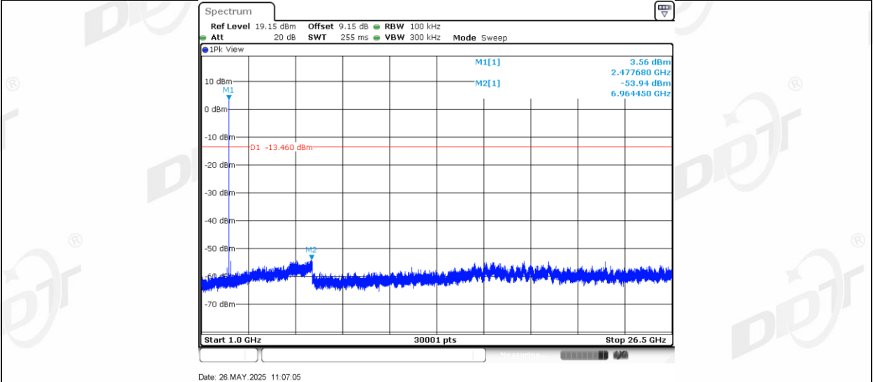
BLE_2M_Right side_2478_0~Reference
