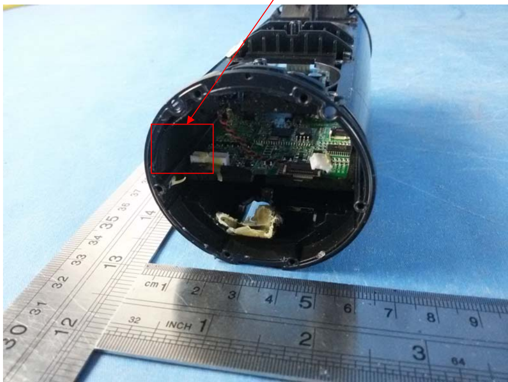
Photo 20 antenna position
