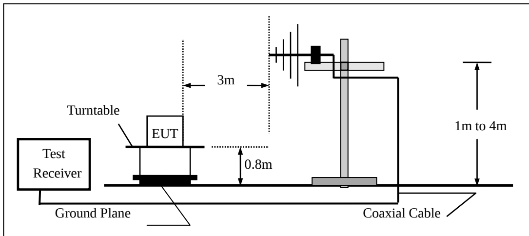
(b) For radiated emissions from 30MHz to 1000MHz
