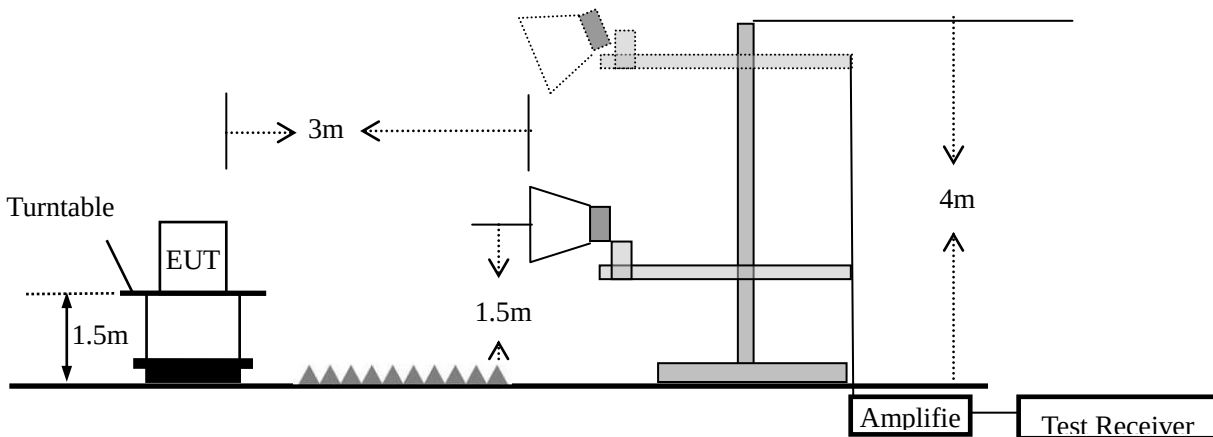
(c) For radiated emissions above 1000MHz
