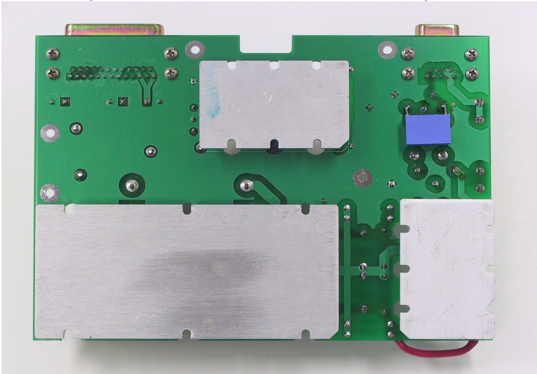
Power Supply
