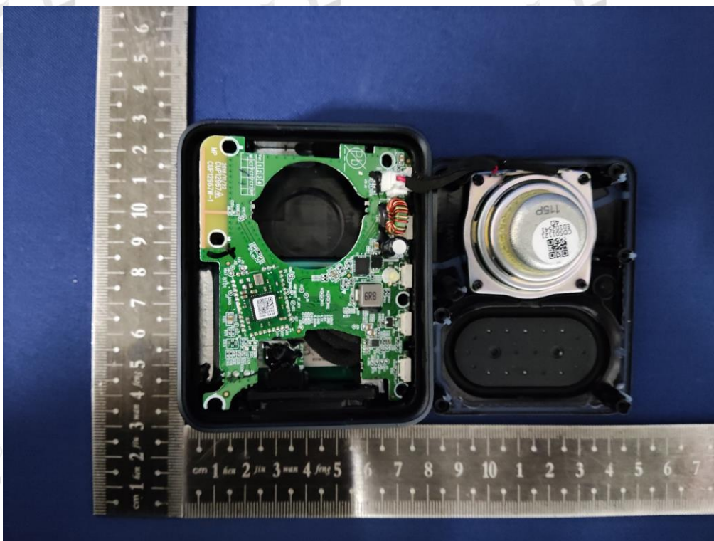
AMP IC: LM48511SQ
