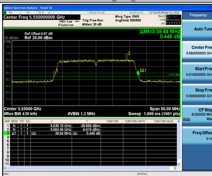
11AC40MIMO Ant2 5550
