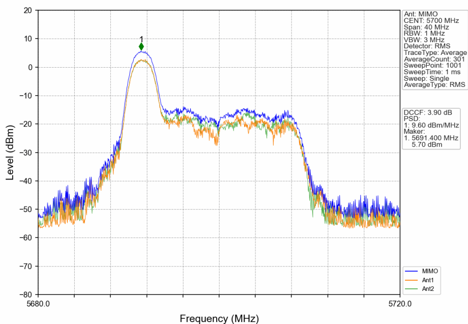
802.11ax(HEW20)_HCH_5700MHz_RU26_Left_MIMO_NTNV
