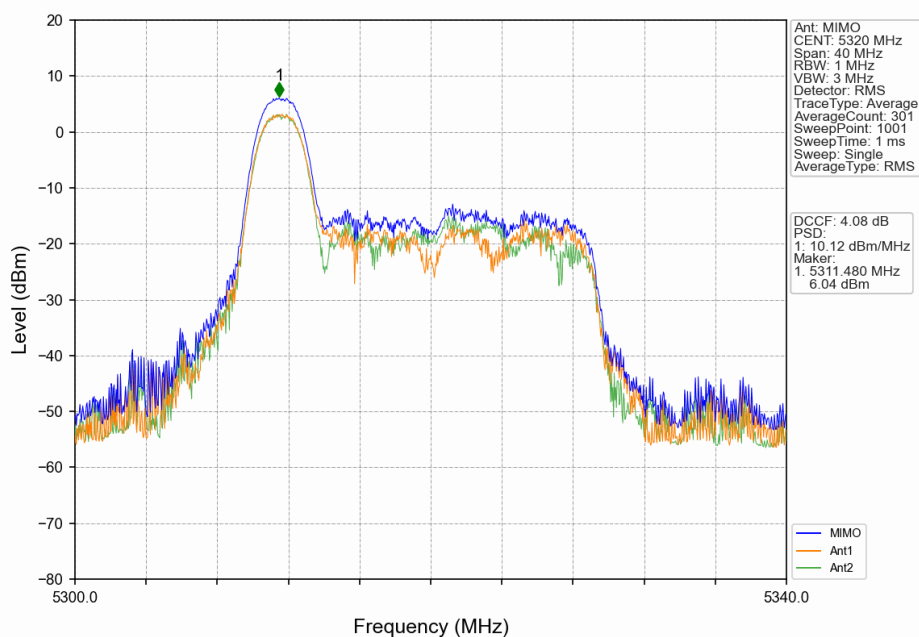
802.11ax(HEW20)_HCH_5320MHz_RU26_Left_MIMO_NTNV
