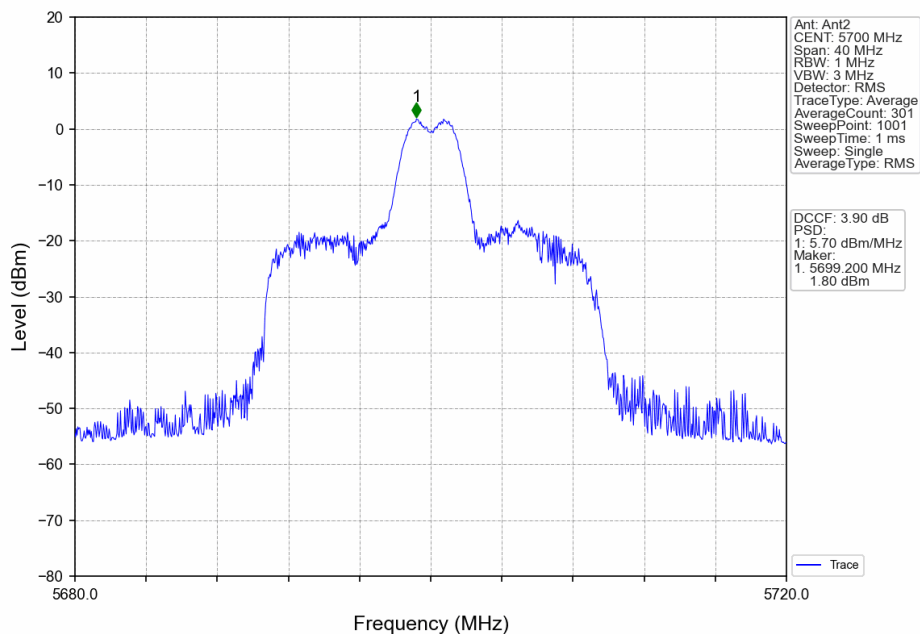
802.11ax(HEW20)_HCH_5700MHz_RU26_Mid_Ant2_NTNV
