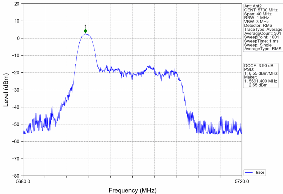
802.11ax(HEW20)_HCH_5700MHz_RU26_Left_MIMO_NTNV
