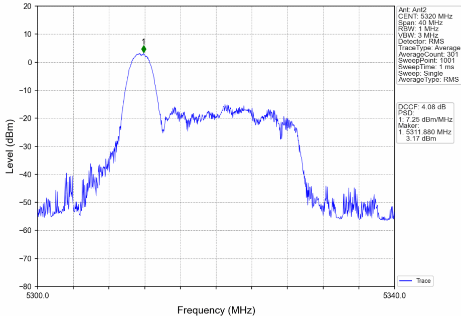
802.11ax(HEW20)_HCH_5320MHz_RU26_Left_MIMO_NTNV
