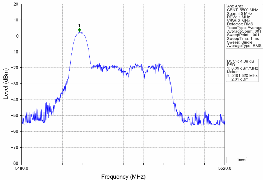
802.11ax(HEW20)_LCH_5500MHz_RU26_Left_MIMO_NTNV
