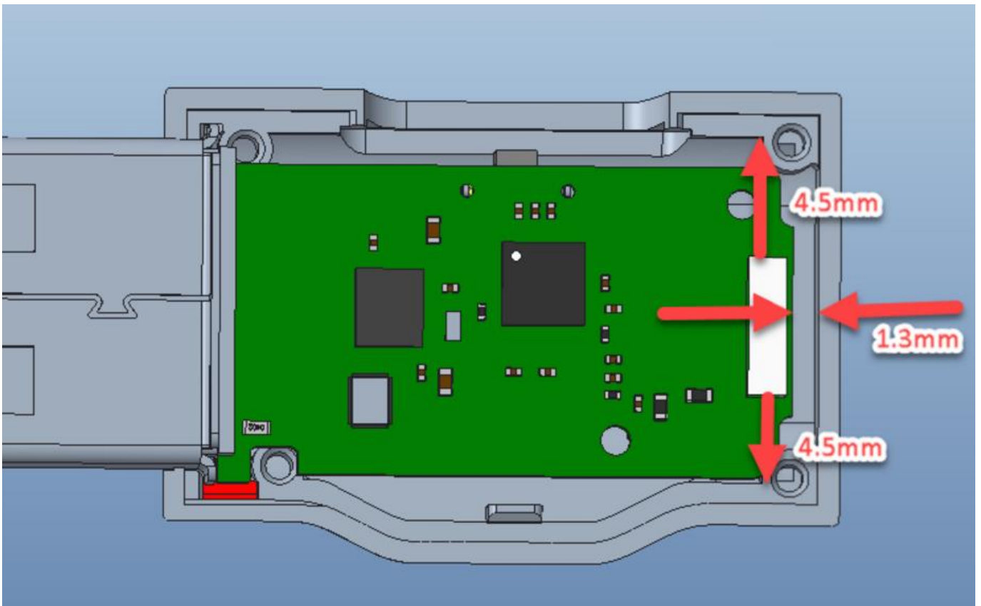
Antenna location diagram
