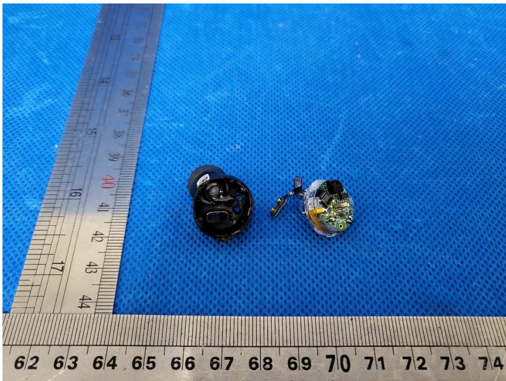
Internal view of right earbud-2
