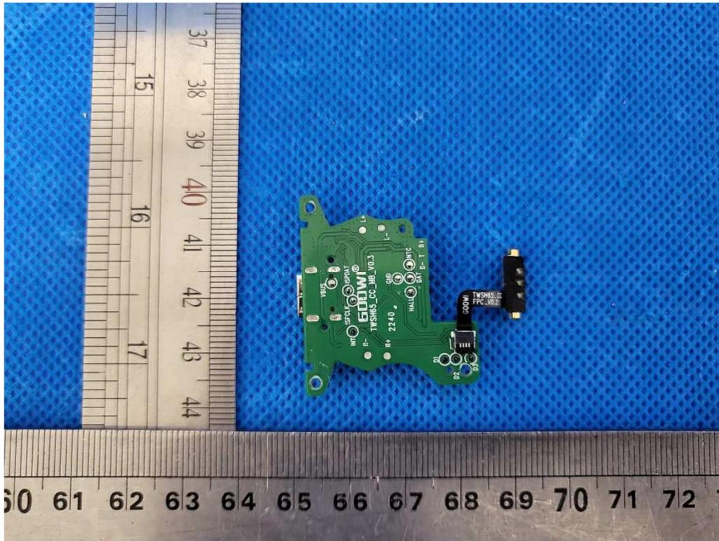
Main board bottom view (charging case)
