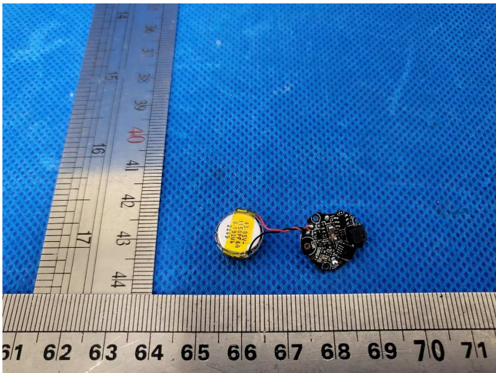
Mainboard and battery view of left earbud-2
