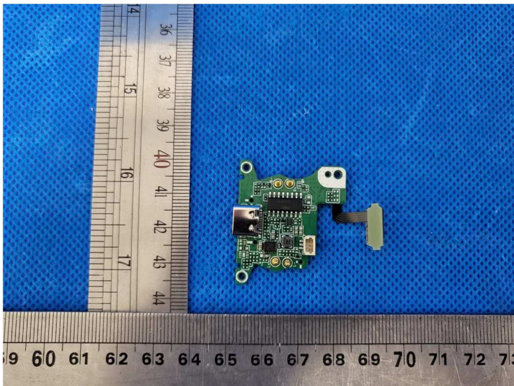
Main board top view (charging case)
