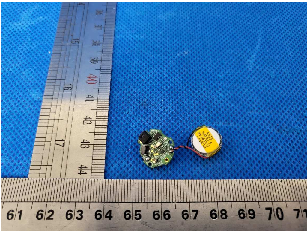
Mainboard and battery view of right earbud-2
