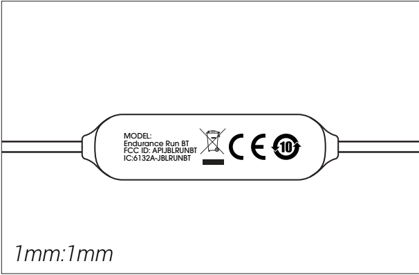
Battery Housing
