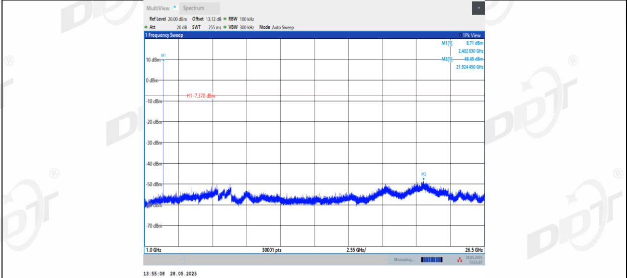
2DH5_Right side_2402_0~Reference
