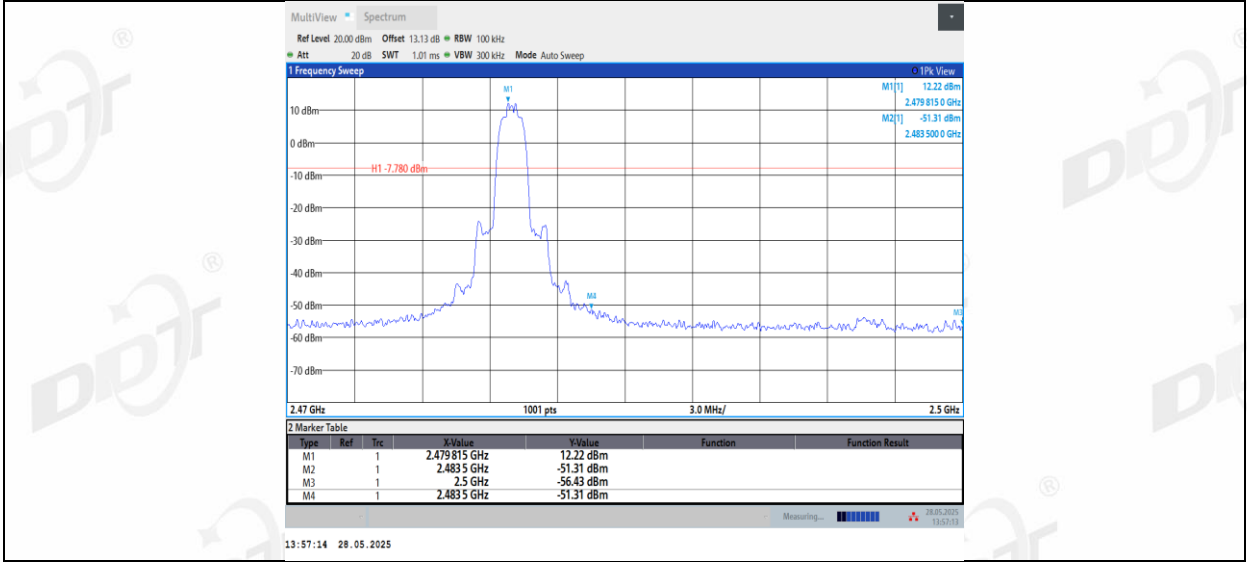
2DH5_Right side_High_2480
