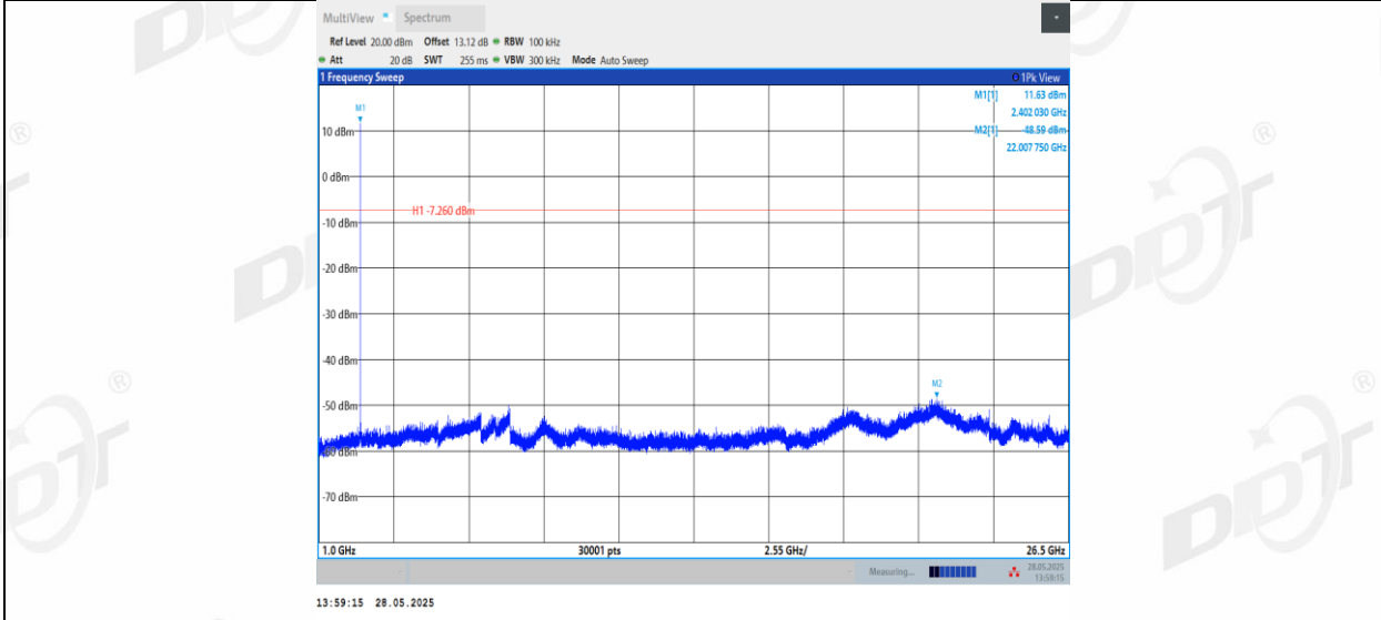
3DH5_Right side_2402_0~Reference
