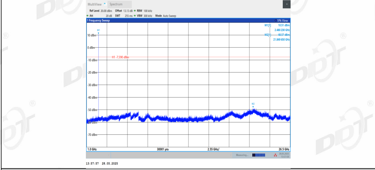
2DH5_Right side_2480_0~Reference
