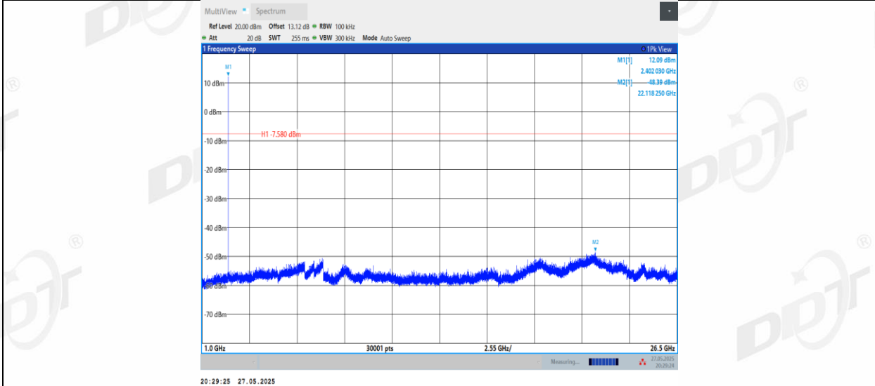
3DH5_Left side_2441_0~Reference
