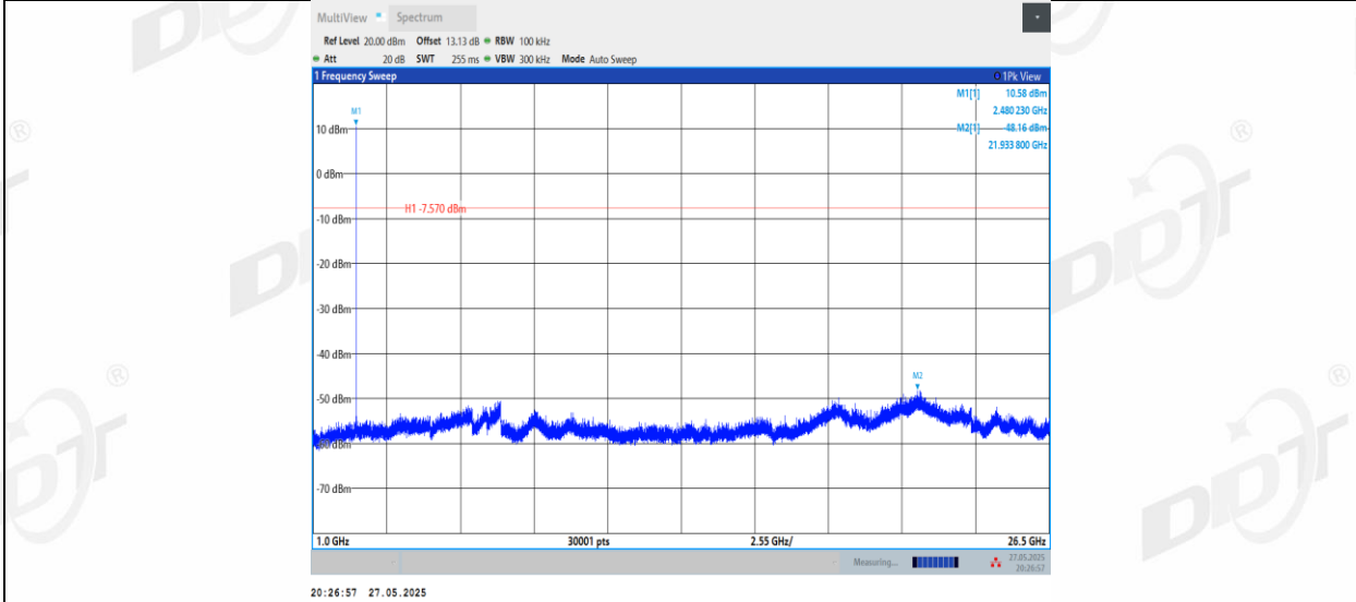
3DH5_Left side_2402_0~Reference
