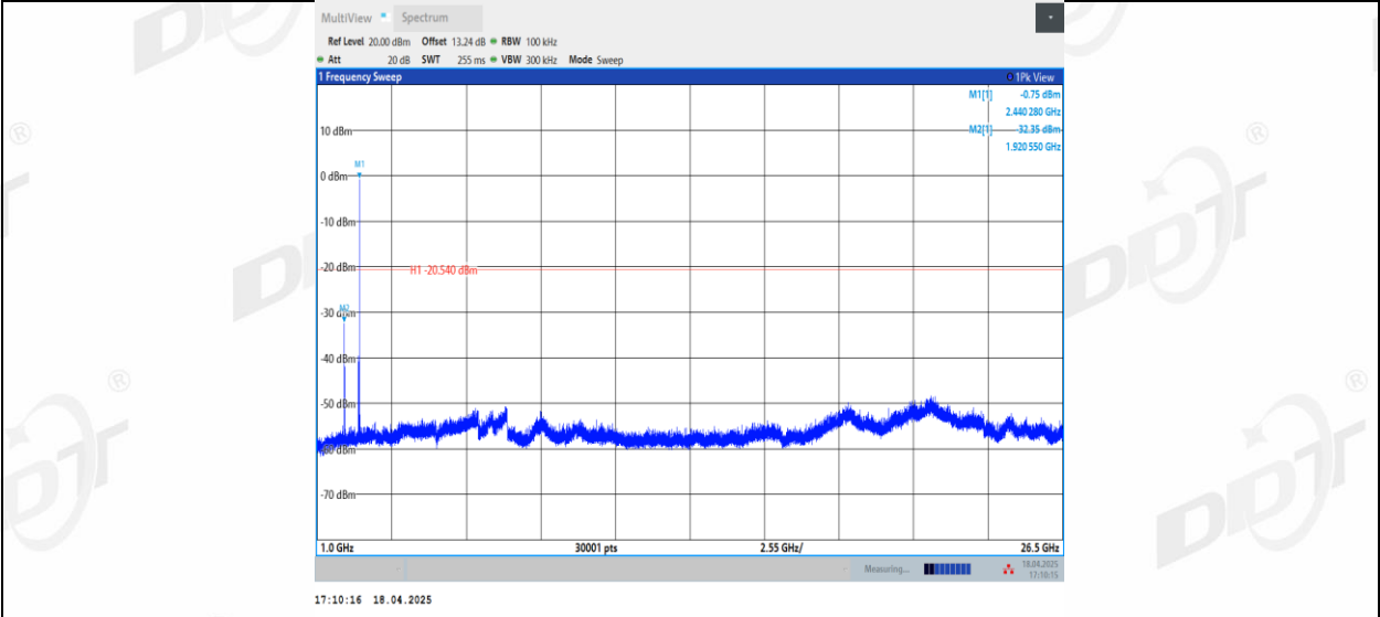
BLE_2M_Ant1_2480_0~Reference
