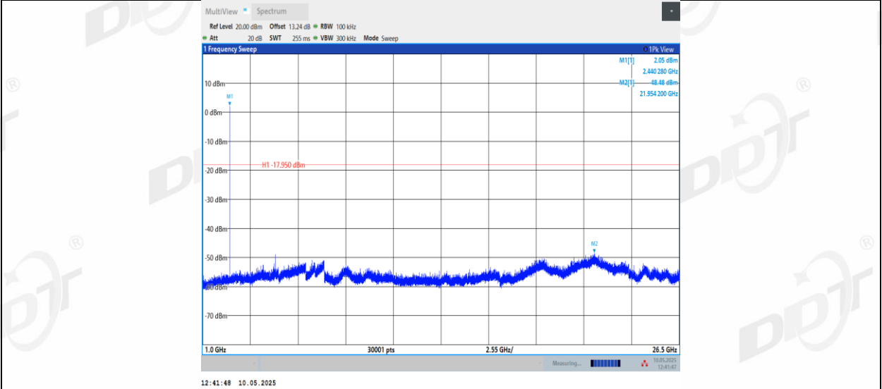
BLE_2M_Ant1_2478_0~Reference
