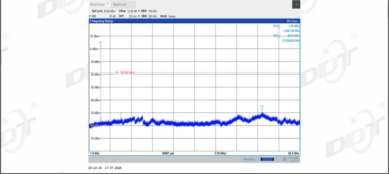
BLE_2M_Ant1_2440_0~Reference
