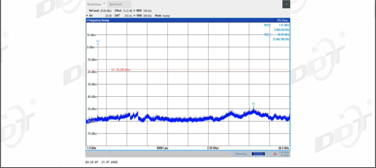
BLE_2M_Ant1_2404_0~Reference
