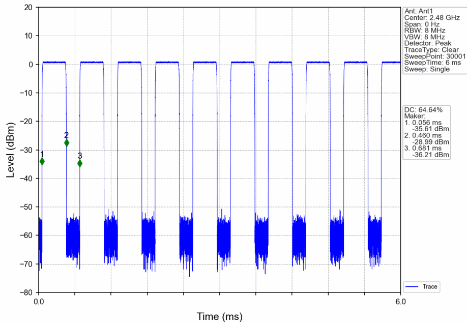
1M_HCH_2480MHz_Ant1_NTNV
