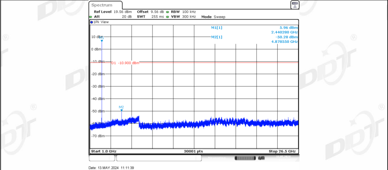
BLE_2M_Right side_2440_0~Reference
