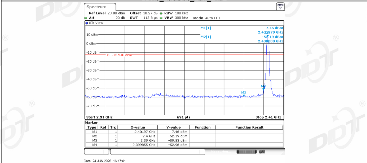
2DH5_Right side_Low_2402
