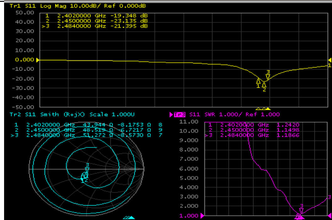
Return loss figure
