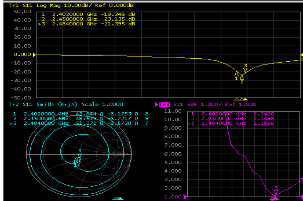
VSWR figure
